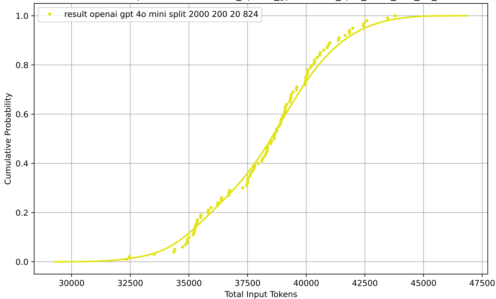
CDF of Total Input Tokens for result_openai_gpt-4o-mini_split_2000_200_20_824
