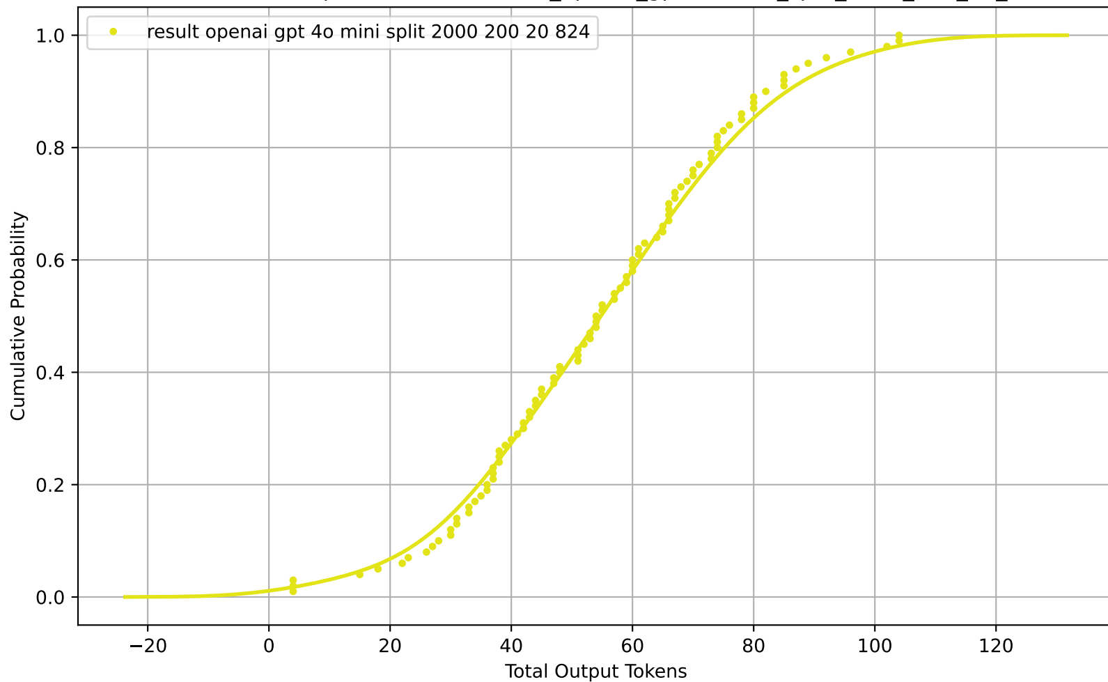
CDF of Total Output Tokens for result_openai_gpt-4o-mini_split_2000_200_20_824
