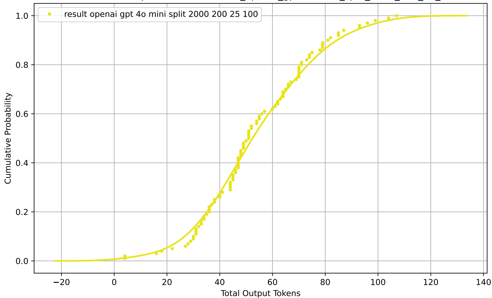
CDF of Total Output Tokens for result_openai_gpt-4o-mini_split_2000_200_25_100
