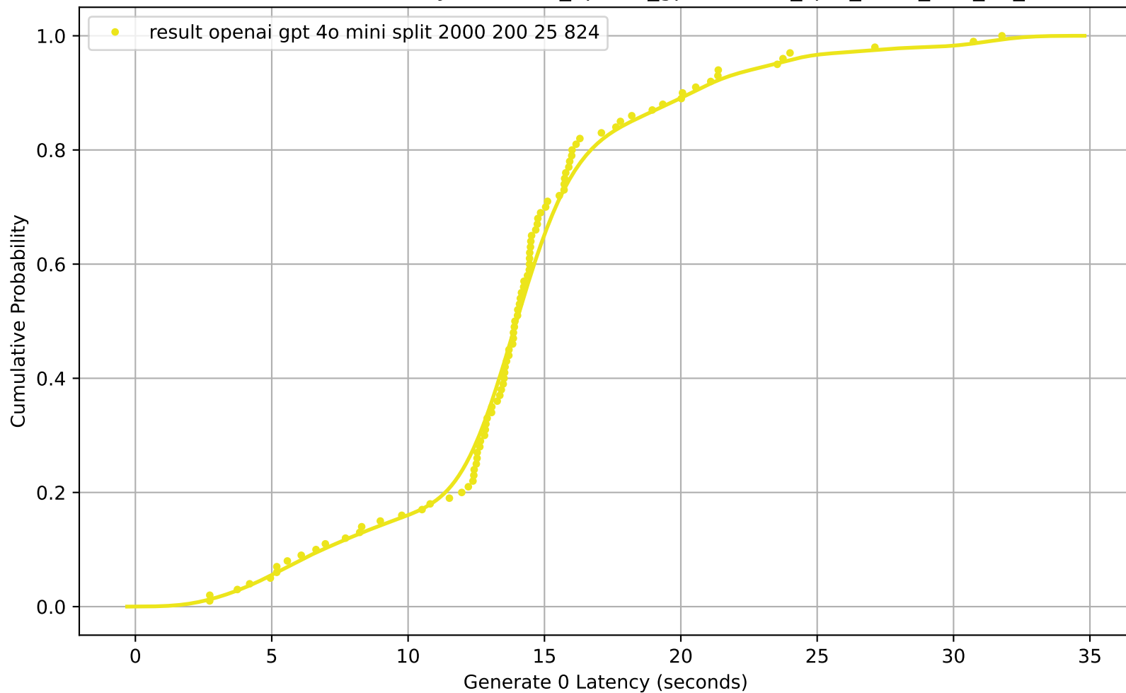
CDF of Generate 0 Latency for result_openai_gpt-4o-mini_split_2000_200_25_824
