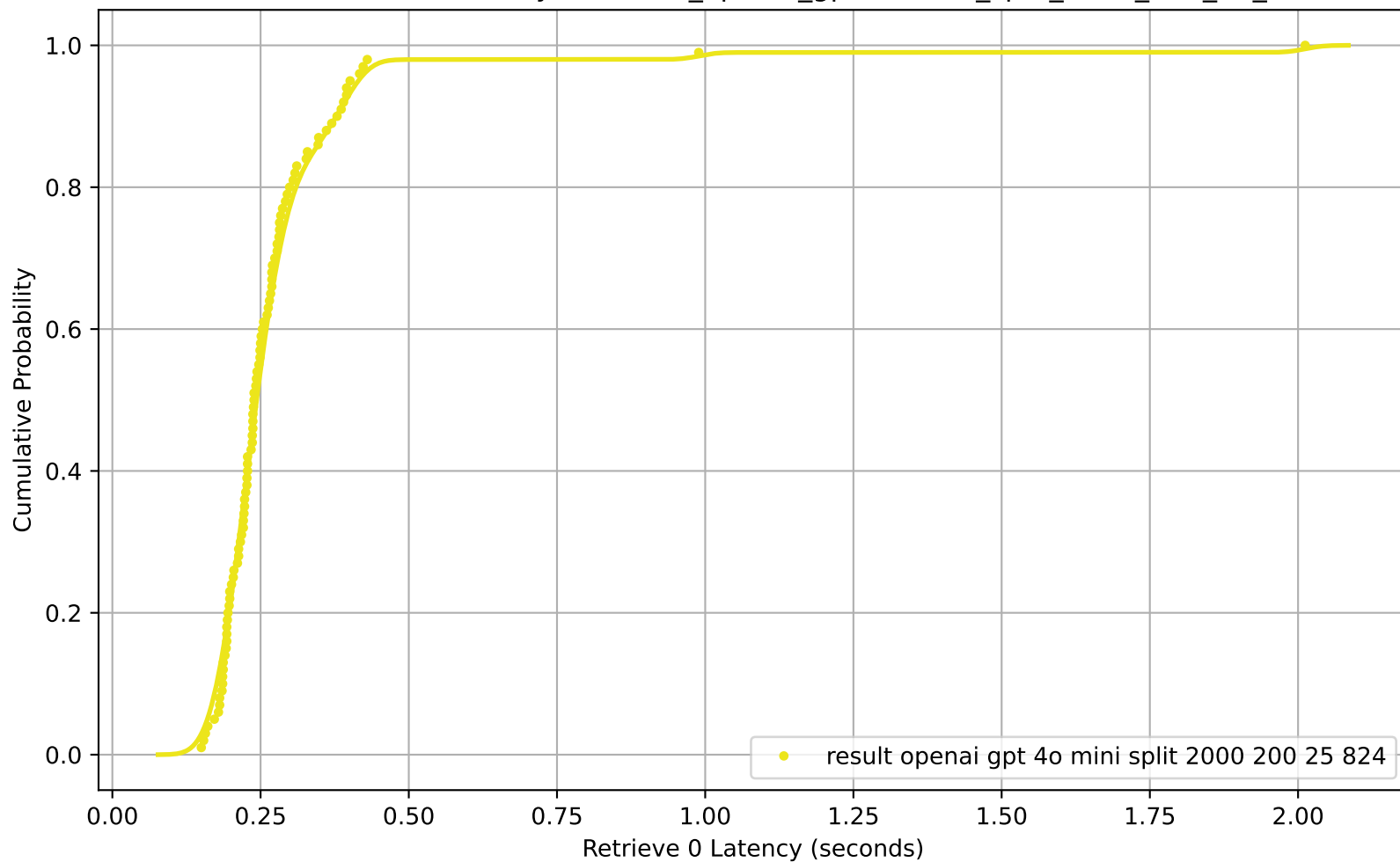
CDF of Retrieve 0 Latency for result_openai_gpt-4o-mini_split_2000_200_25_824
