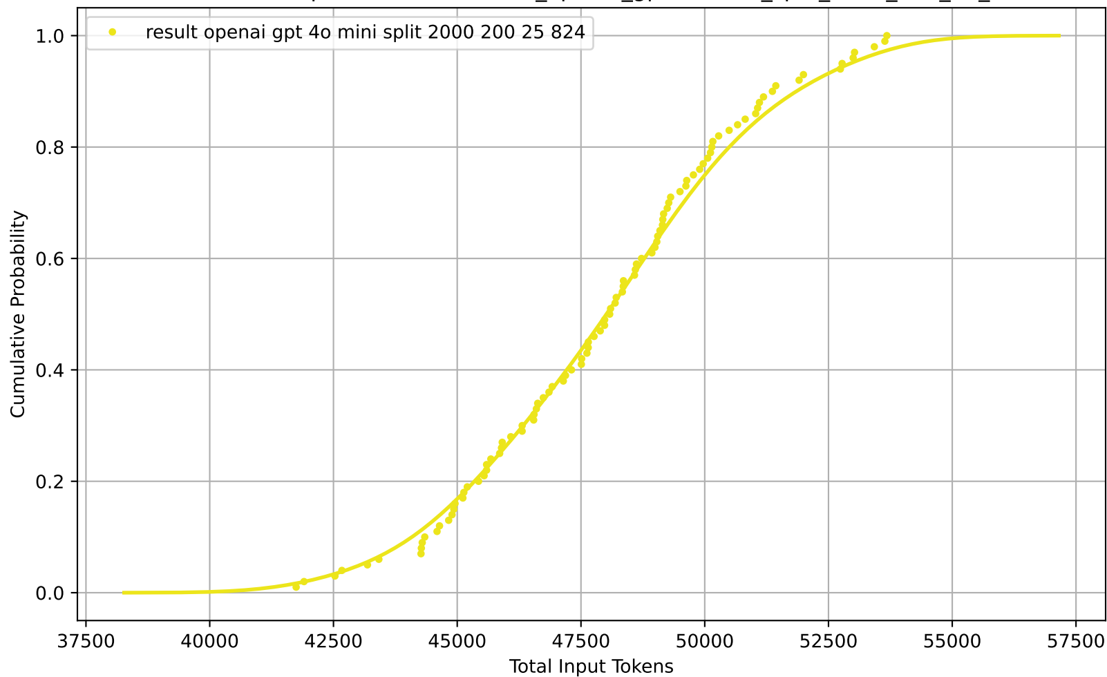
CDF of Total Input Tokens for result_openai_gpt-4o-mini_split_2000_200_25_824
