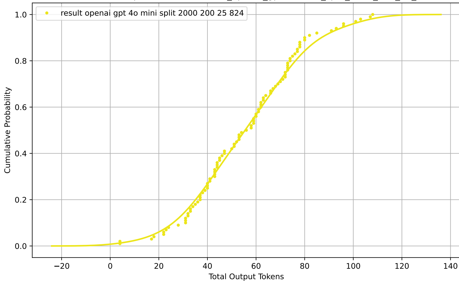
CDF of Total Output Tokens for result_openai_gpt-4o-mini_split_2000_200_25_824
