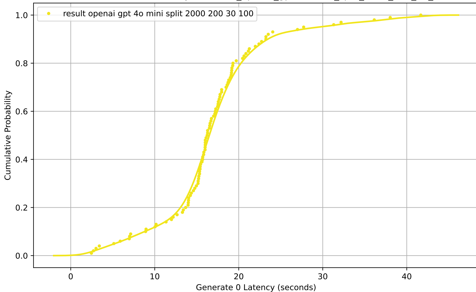
CDF of Generate 0 Latency for result_openai_gpt-4o-mini_split_2000_200_30_100
