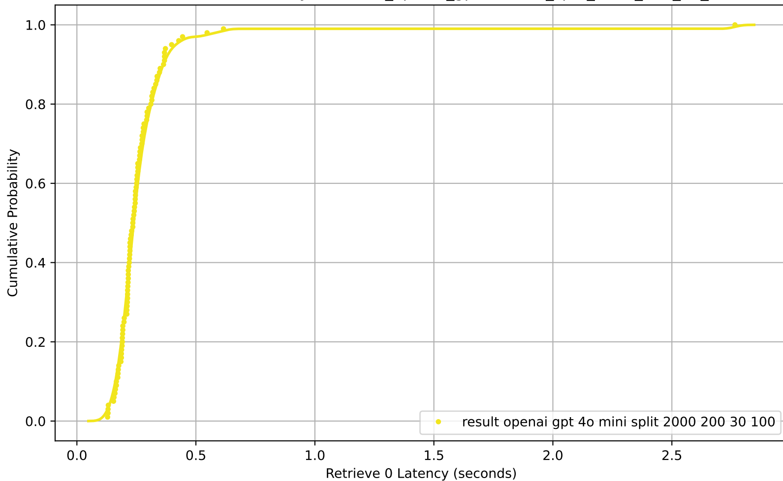
CDF of Retrieve 0 Latency for result_openai_gpt-4o-mini_split_2000_200_30_100
