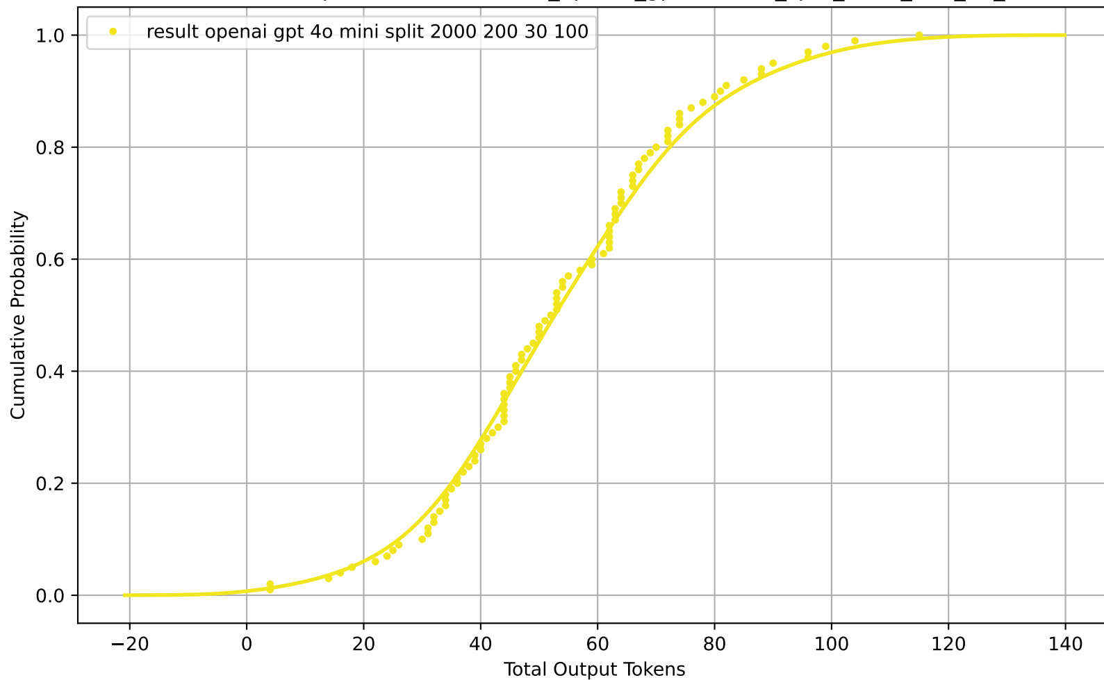
CDF of Total Output Tokens for result_openai_gpt-4o-mini_split_2000_200_30_100
