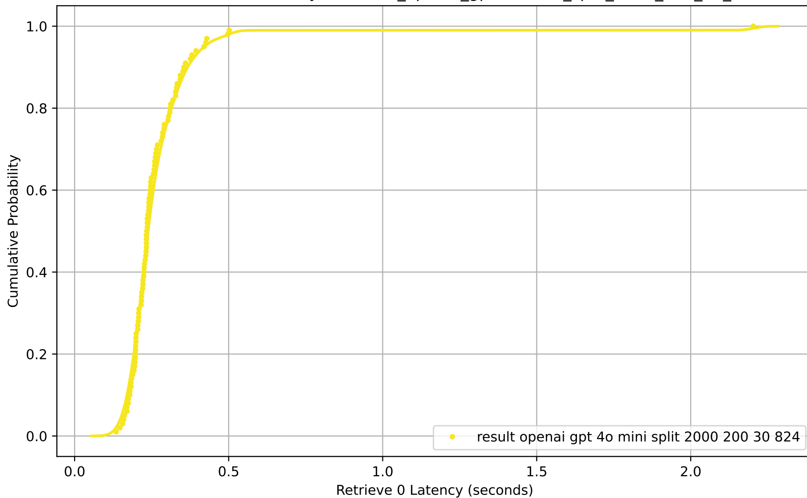
CDF of Retrieve 0 Latency for result_openai_gpt-4o-mini_split_2000_200_30_824
