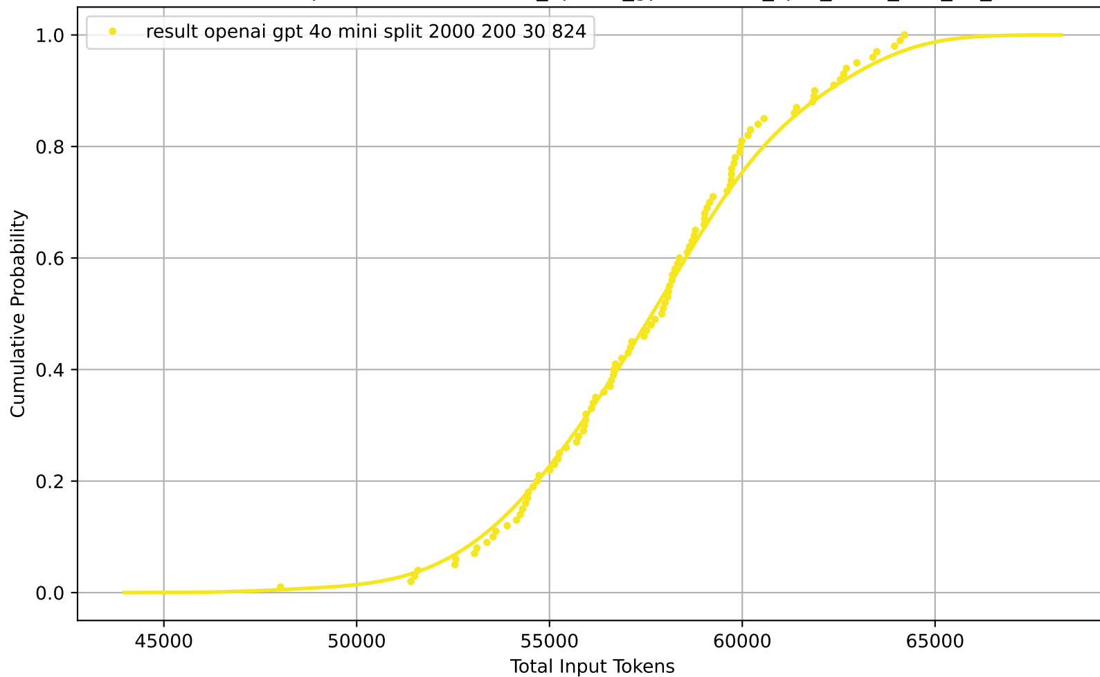
CDF of Total Input Tokens for result_openai_gpt-4o-mini_split_2000_200_30_824
