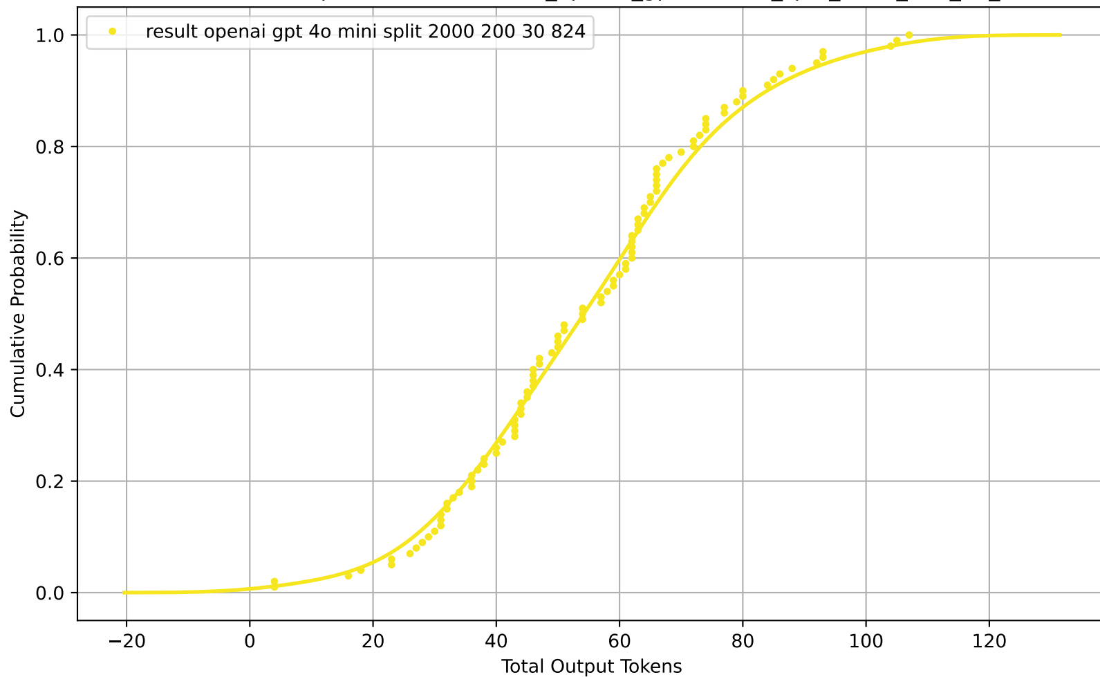
CDF of Total Output Tokens for result_openai_gpt-4o-mini_split_2000_200_30_824
