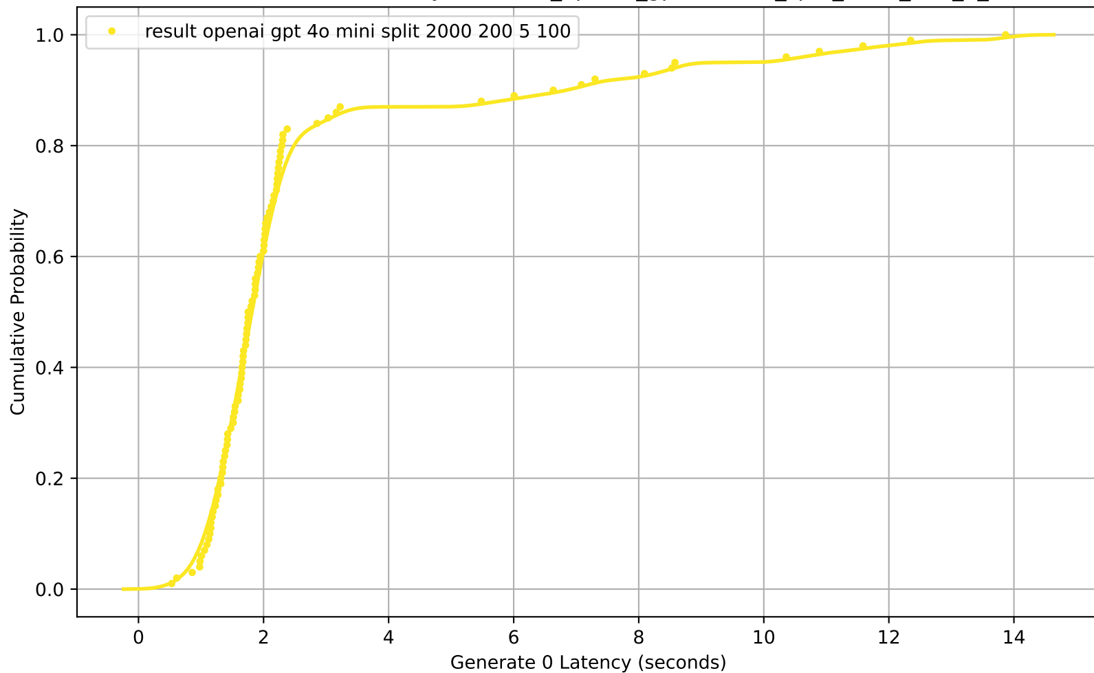
CDF of Generate 0 Latency for result_openai_gpt-4o-mini_split_2000_200_5_100
