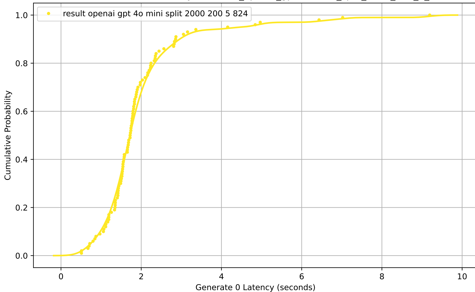
CDF of Generate 0 Latency for result_openai_gpt-4o-mini_split_2000_200_5_824
