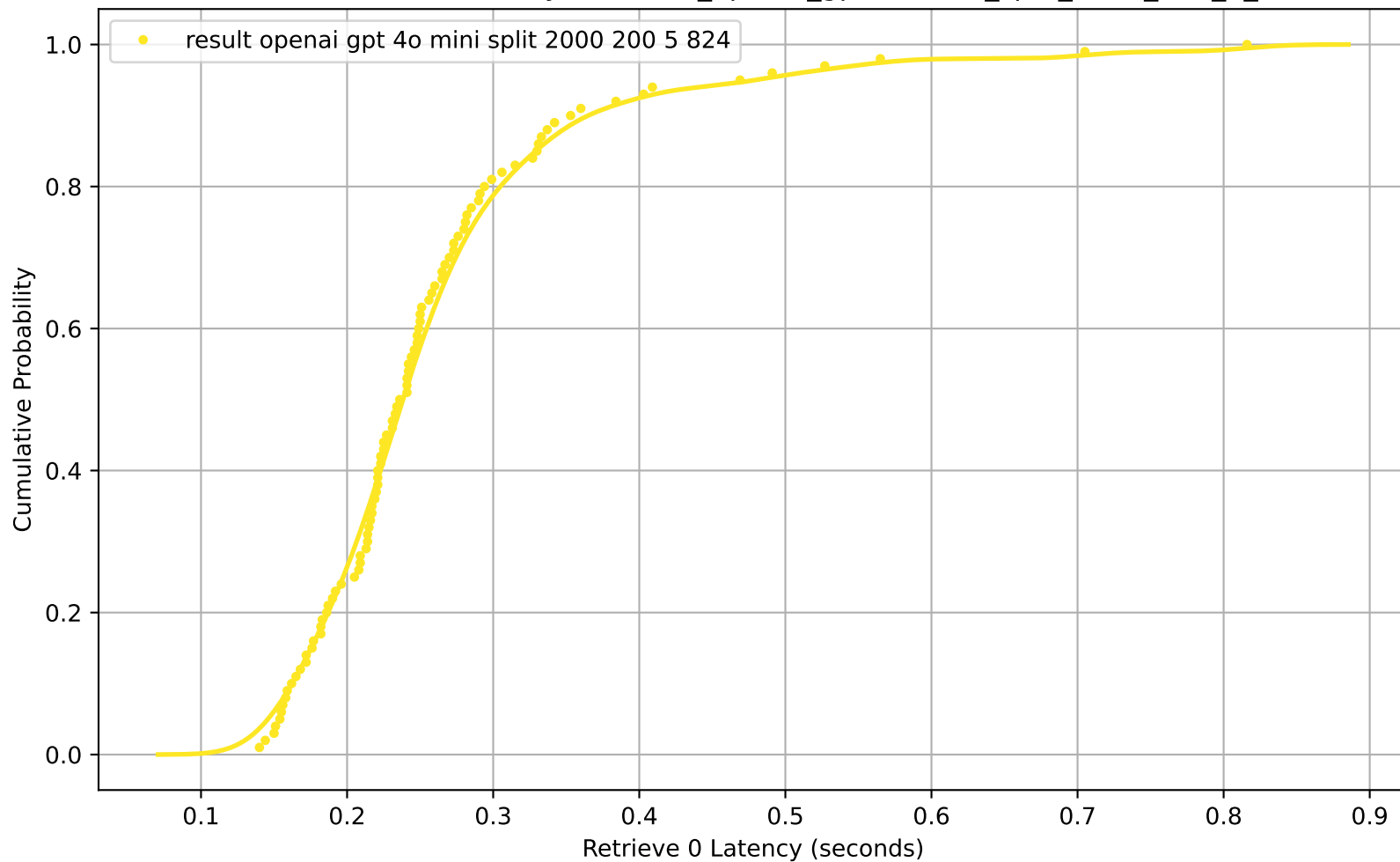
CDF of Retrieve 0 Latency for result_openai_gpt-4o-mini_split_2000_200_5_824
