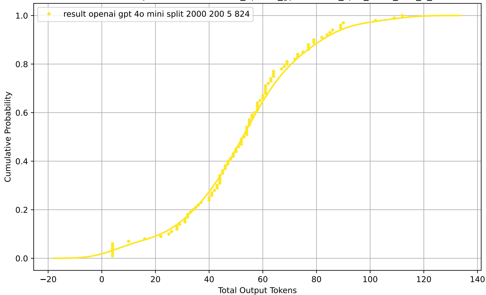
CDF of Total Output Tokens for result_openai_gpt-4o-mini_split_2000_200_5_824
