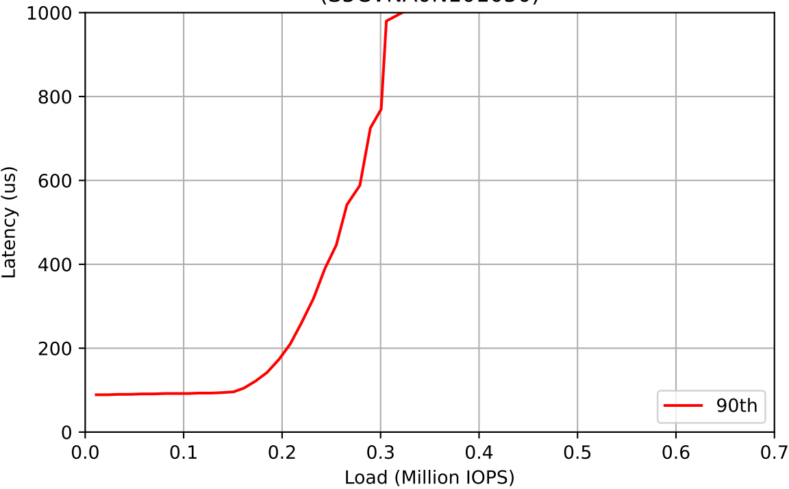
Workload: 700% Writes (S5CVNA0N101050)
