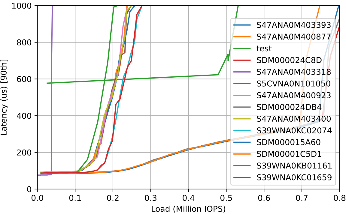
Workload: 500% Writes
