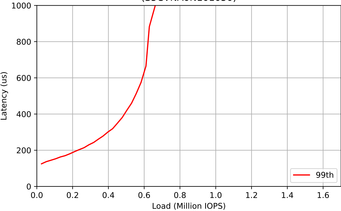
Workload: 100% Reads (S5CVNA0N101050)
