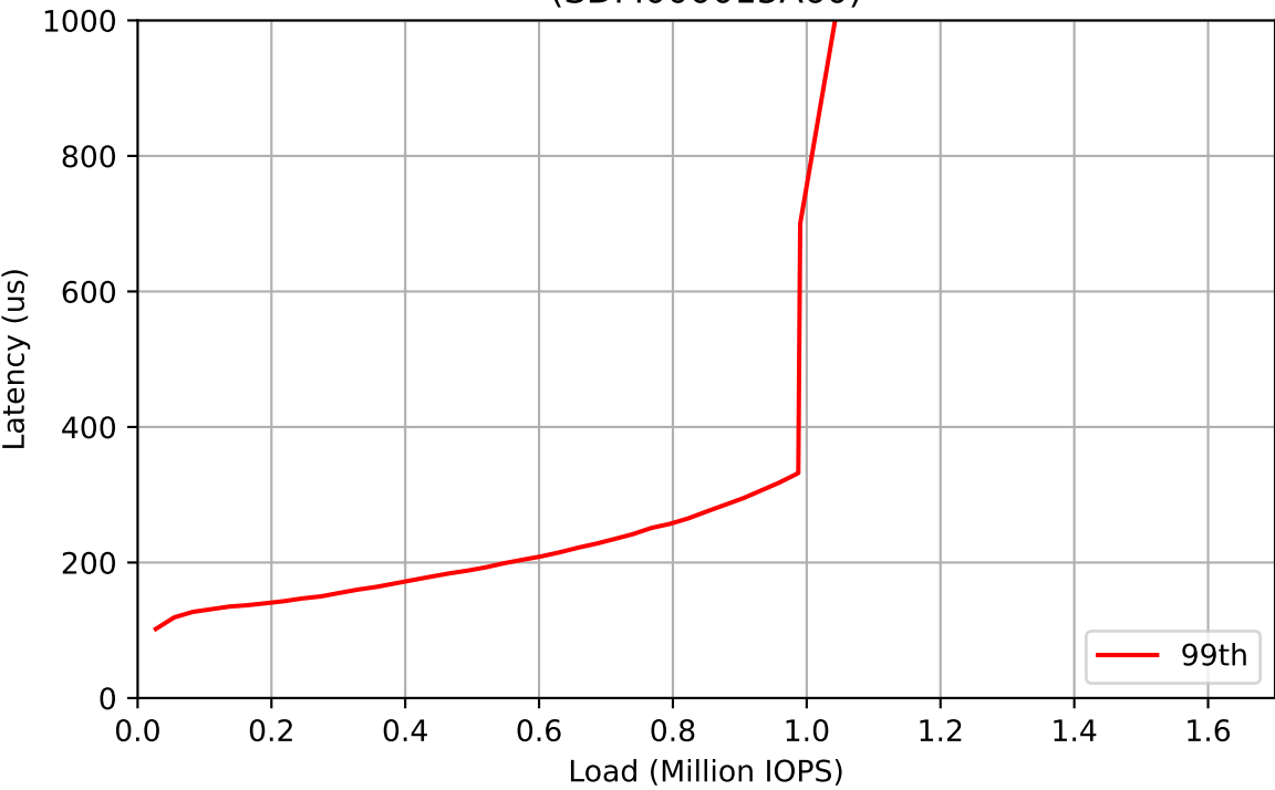
Workload: 100% Reads (SDM000015A60)
