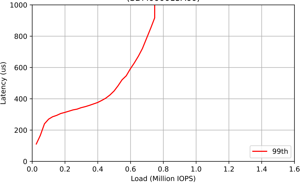
Workload: 250% Writes (SDM000015A60)
