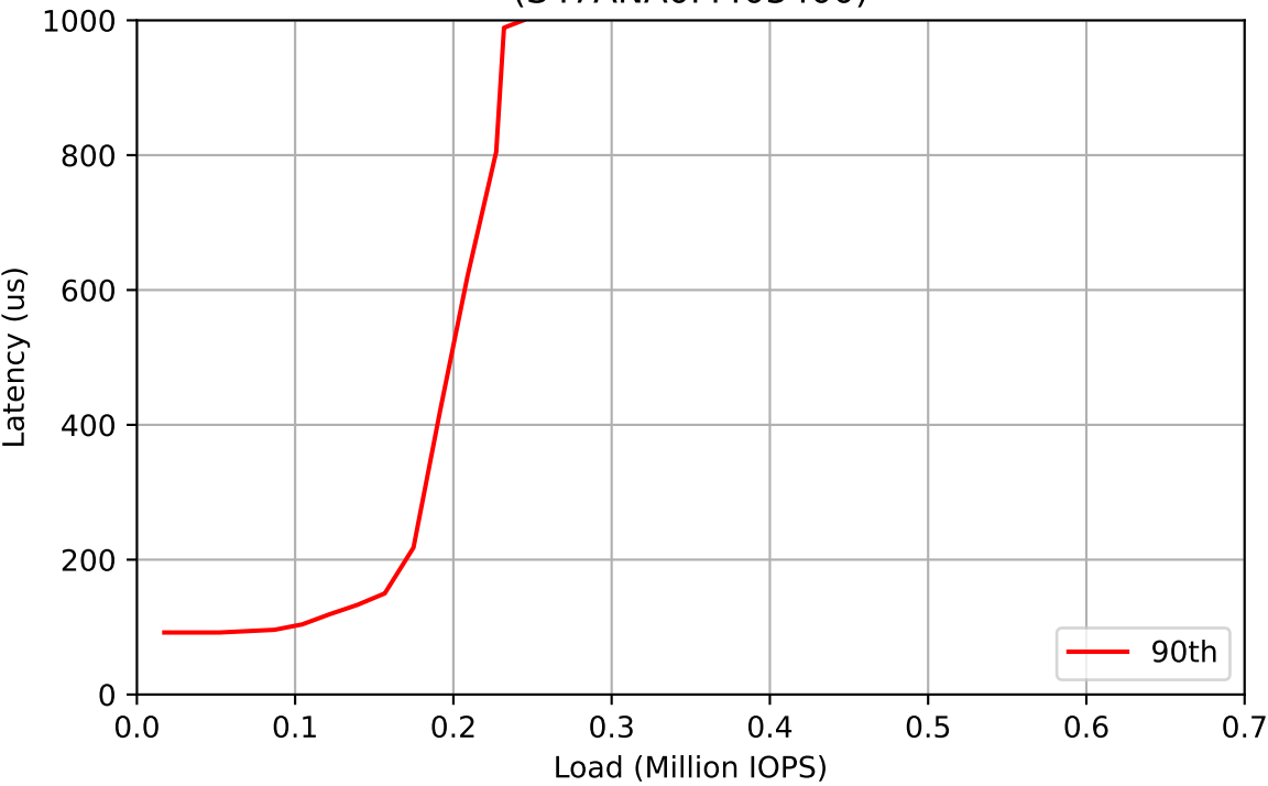
Workload: 250% Writes (S47ANA0M403400)
