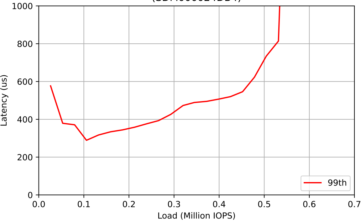
Workload: 500% Writes (SDM000024DB4)
