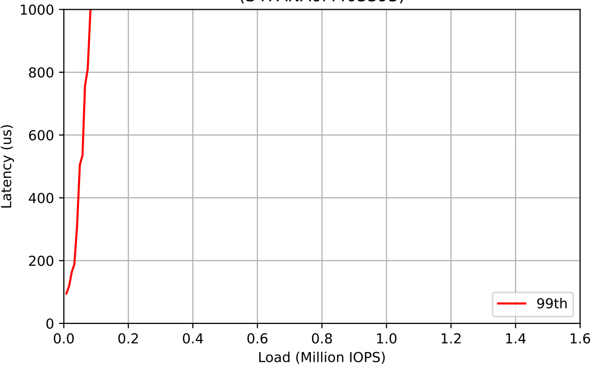
Workload: 300% Writes (S47ANA0M403393)
