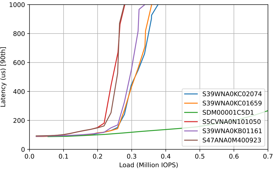
Workload: 100% Writes
