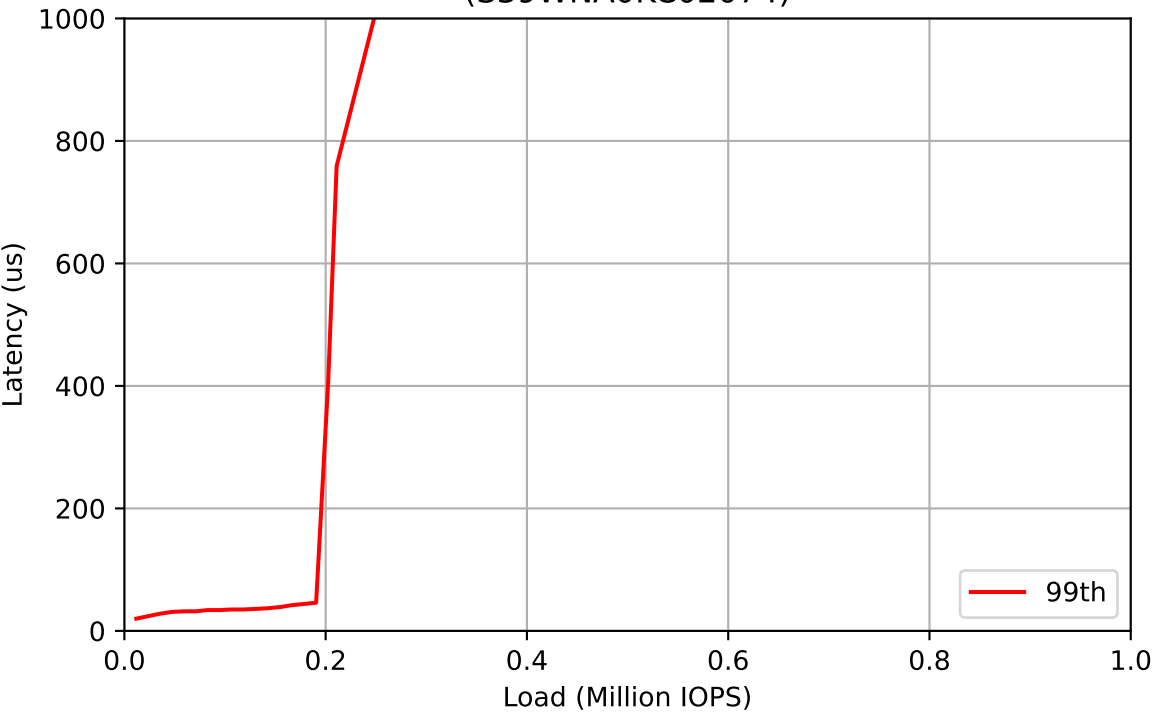
Workload: 1000% Writes (S39WNA0KC02074)
