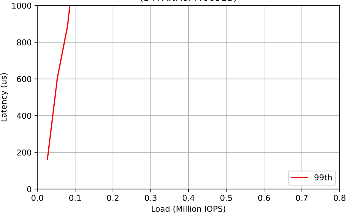
Workload: 500% Writes (S47ANA0M400923)
