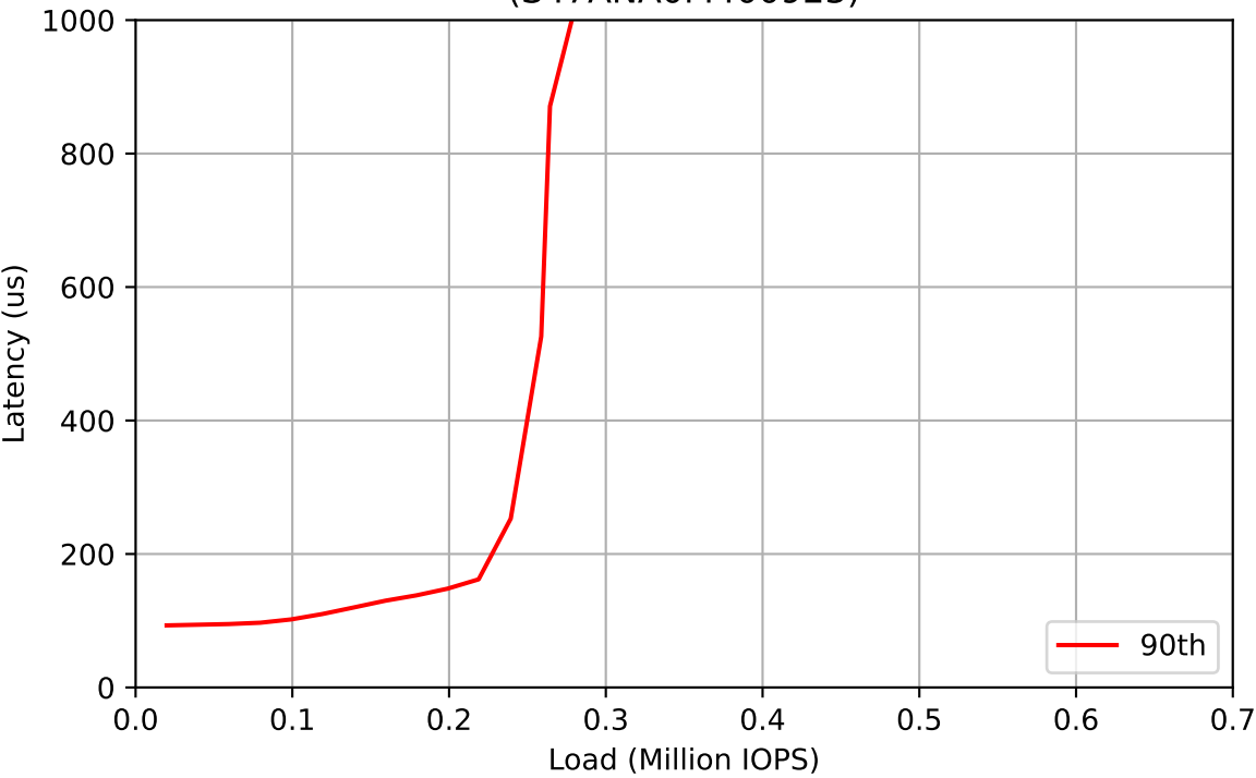
Workload: 100% Writes (S47ANA0M400923)
