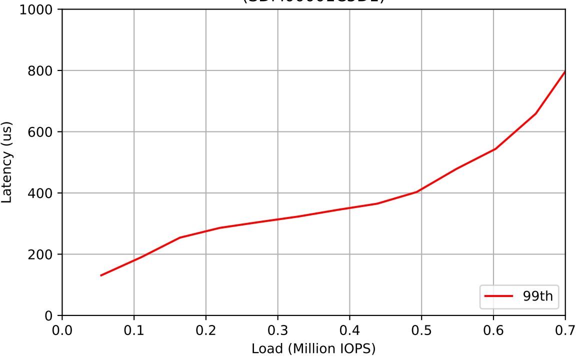
Workload: 100% Writes (SDM00001C5D1)
