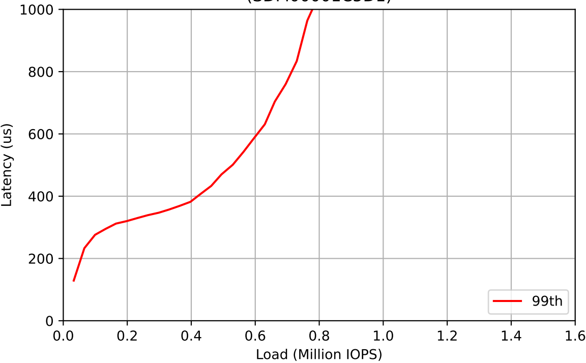
Workload: 300% Writes (SDM00001C5D1)
