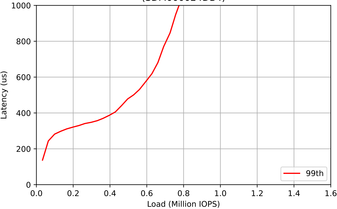
Workload: 300% Writes (SDM000024DB4)
