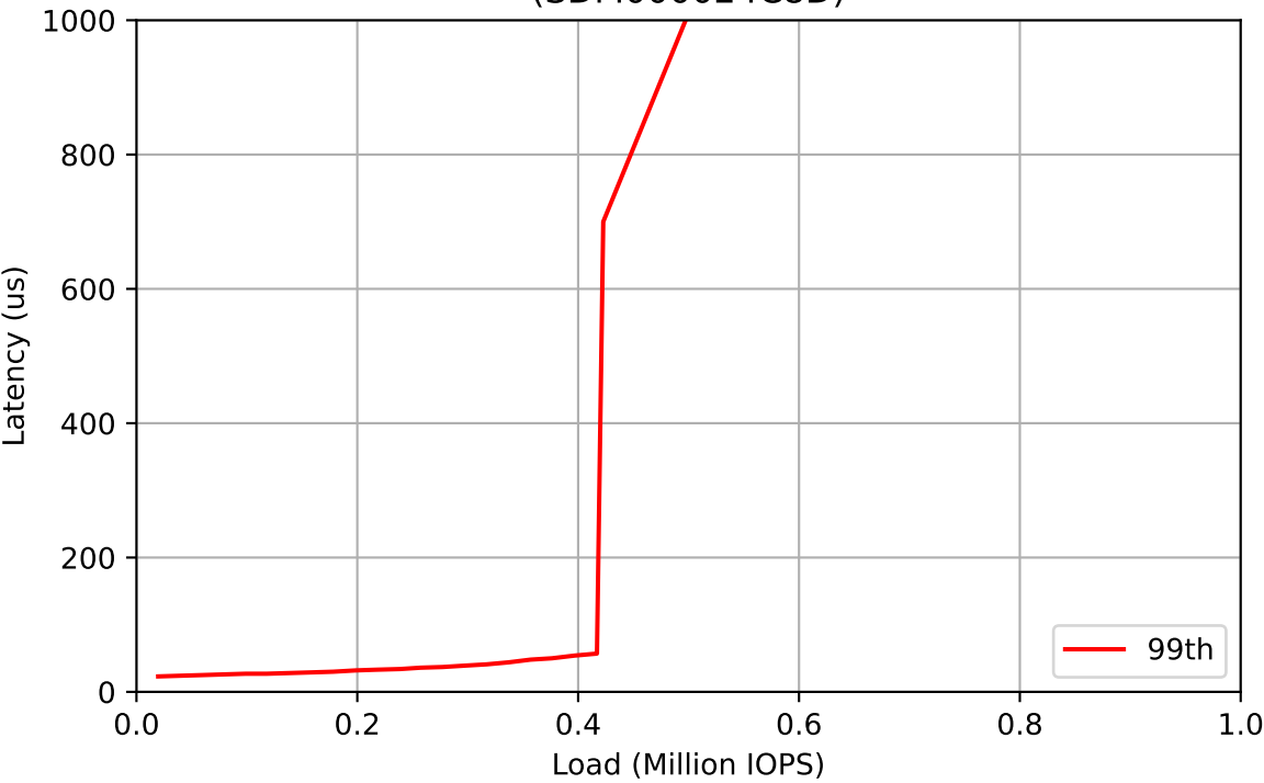
Workload: 1000% Writes (SDM000024C8D)
