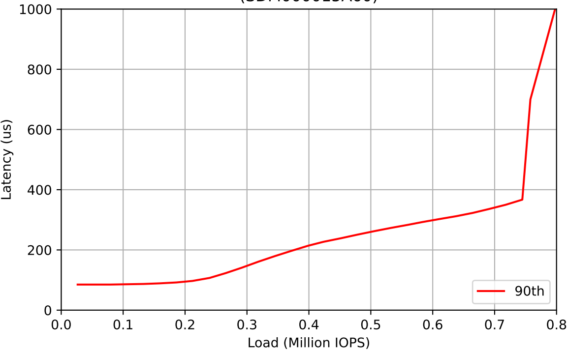
Workload: 500% Writes (SDM000015A60)
