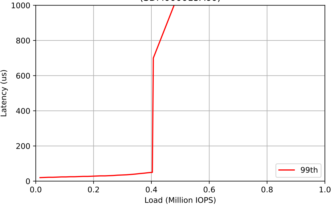
Workload: 1000% Writes (SDM000015A60)
