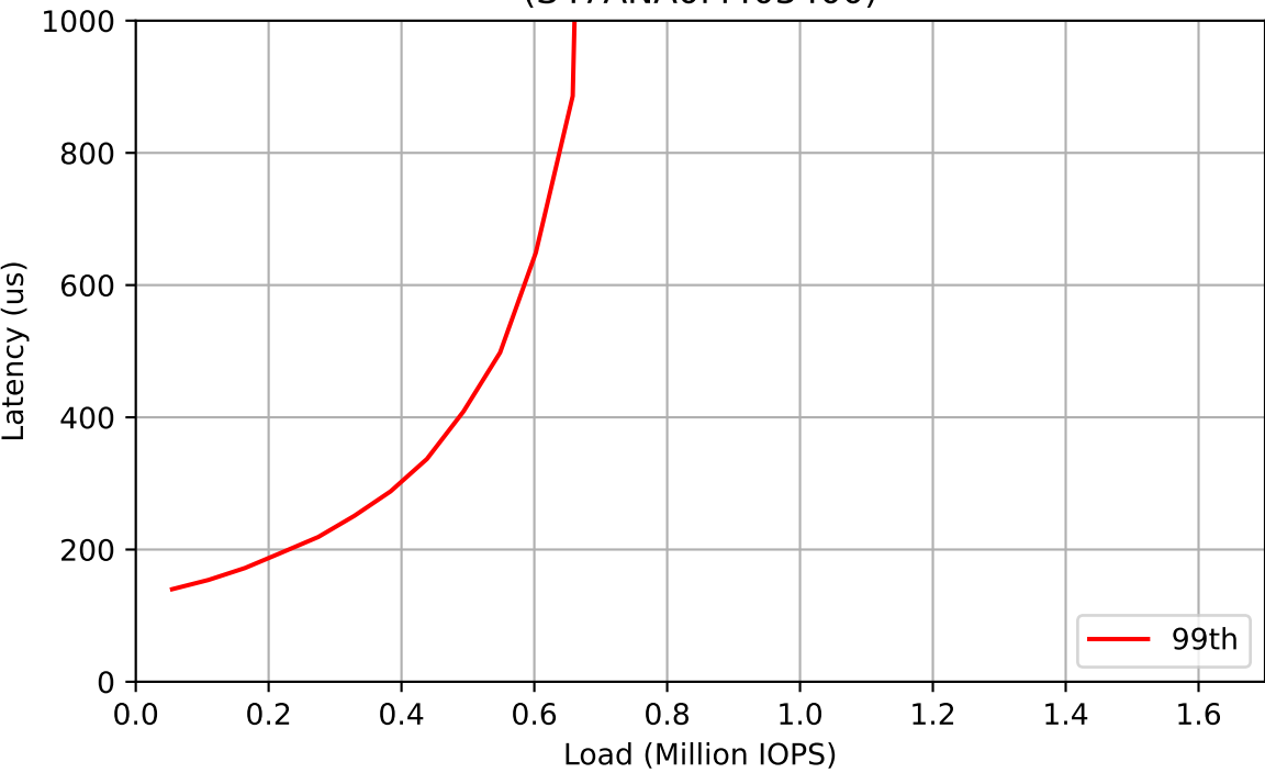
Workload: 100% Reads (S47ANA0M403400)
