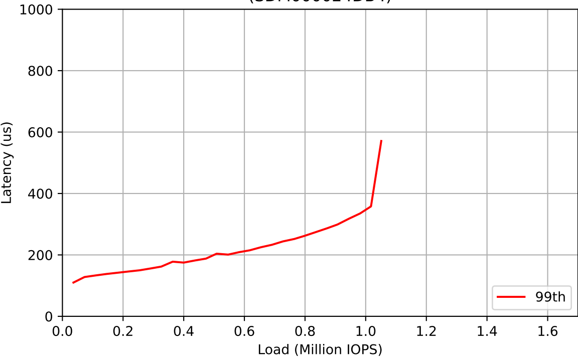
Workload: 100% Reads (SDM000024DB4)
