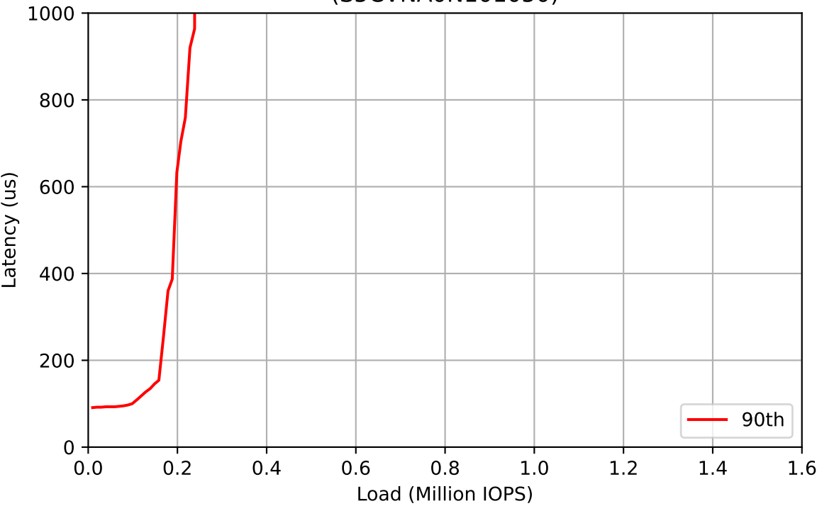
Workload: 300% Writes (S5CVNA0N101050)
