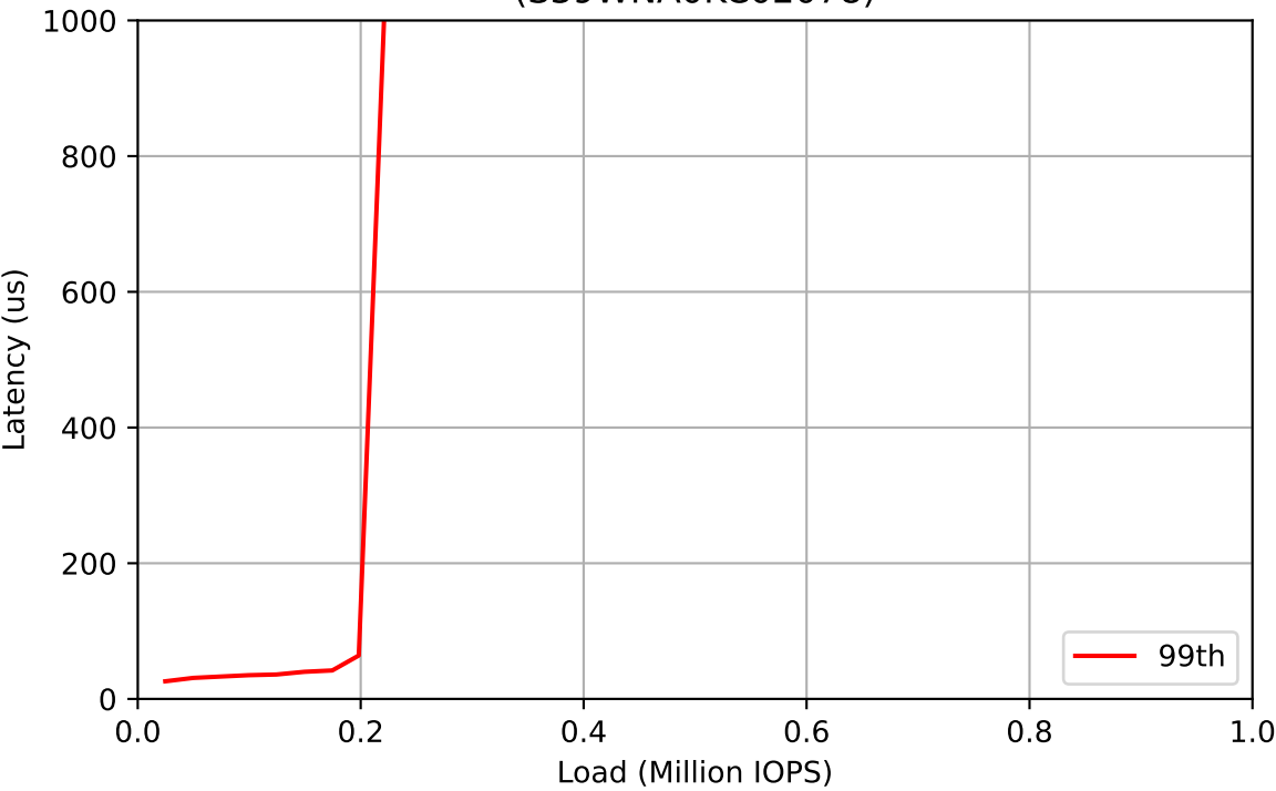
Workload: 1000% Writes (S39WNA0KC02078)
