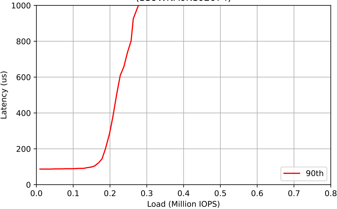
Workload: 500% Writes (S39WNA0KC02074)
