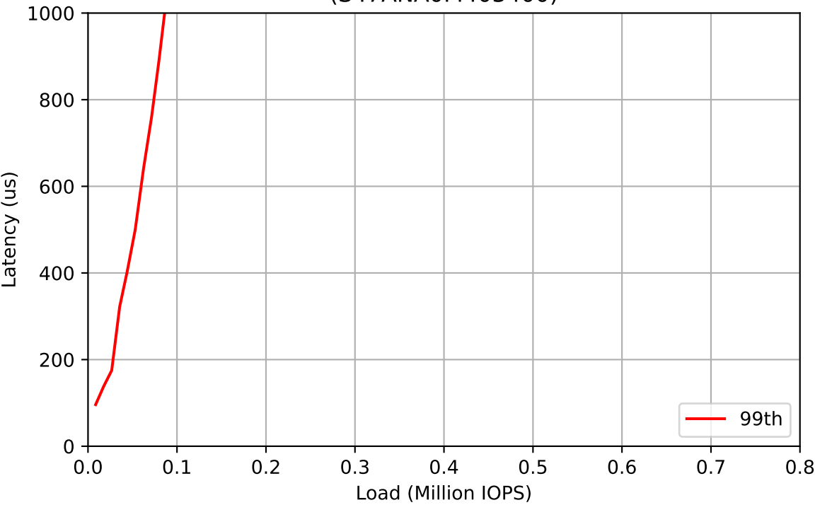
Workload: 500% Writes (S47ANA0M403400)
