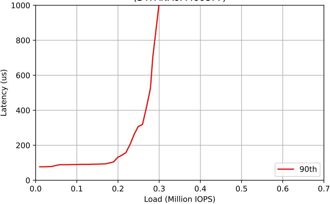
Workload: 750% Writes (S47ANA0M400877)
