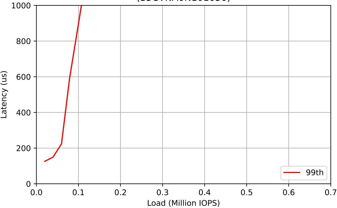
Workload: 100% Writes (S5CVNA0N101050)
