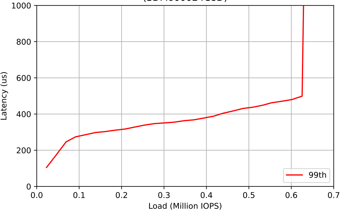
Workload: 700% Writes (SDM000024C8D)
