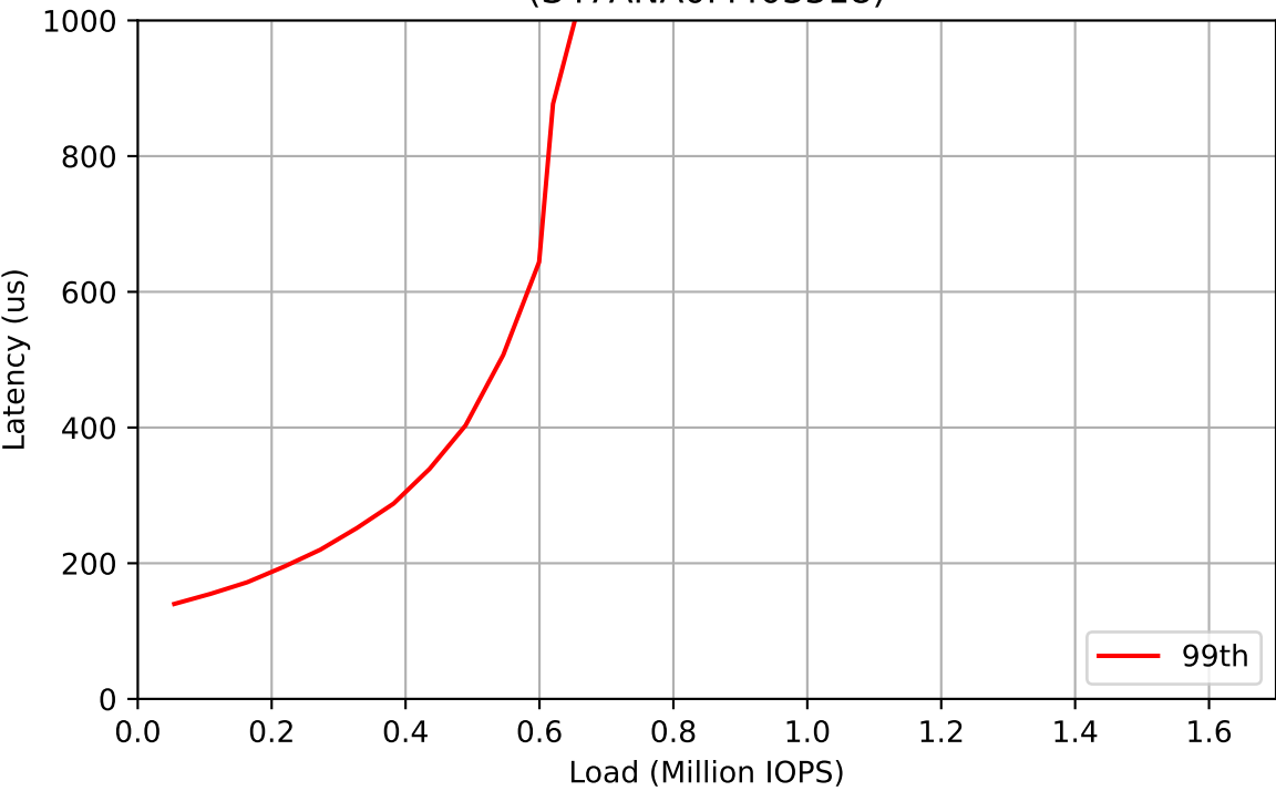
Workload: 100% Reads (S47ANA0M403318)
