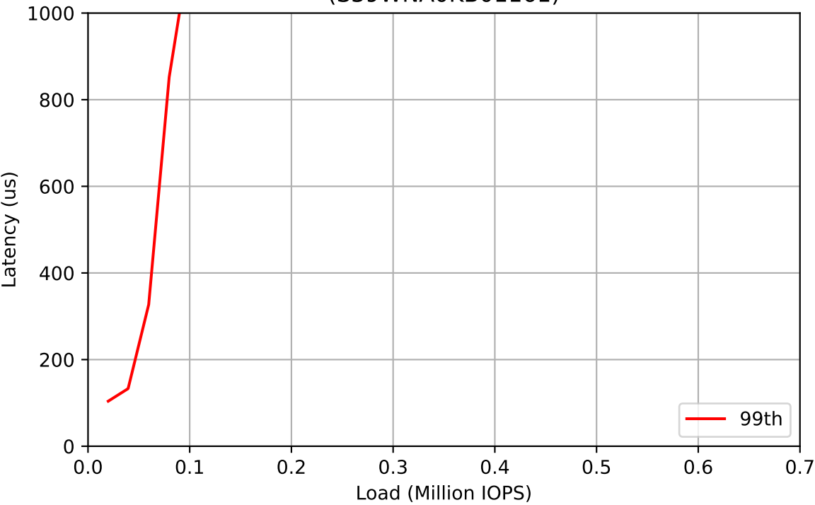
Workload: 100% Writes (S39WNA0KB01161)
