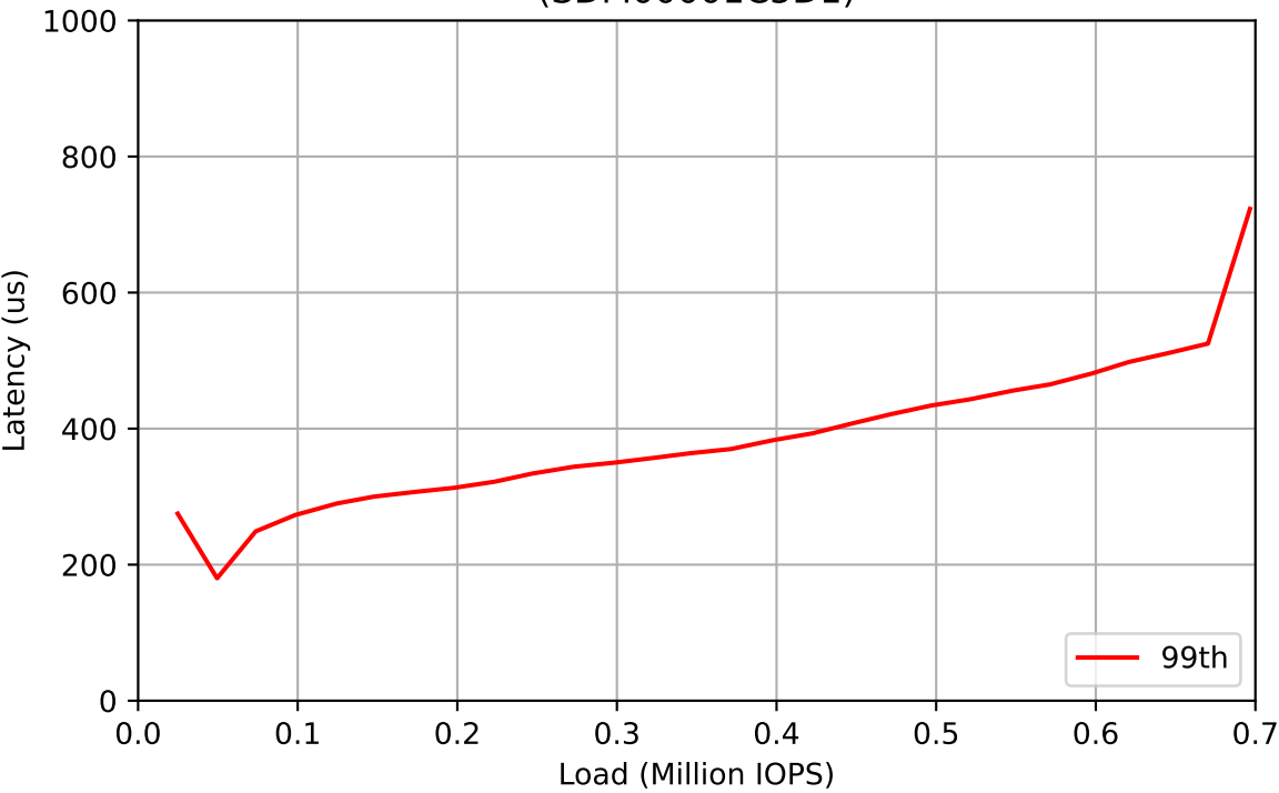
Workload: 700% Writes (SDM00001C5D1)
