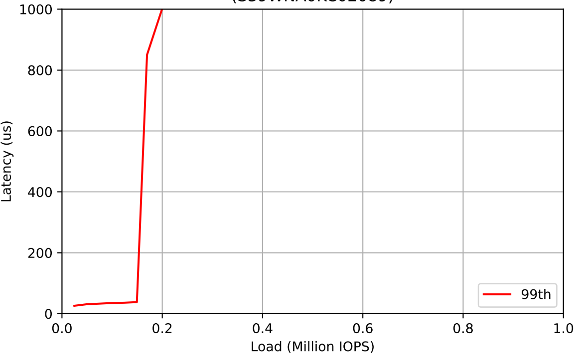
Workload: 1000% Writes (S39WNA0KC02089)
