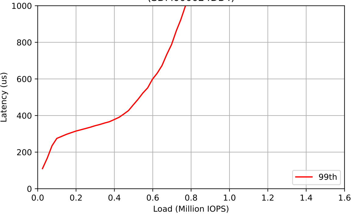
Workload: 250% Writes (SDM000024DB4)
