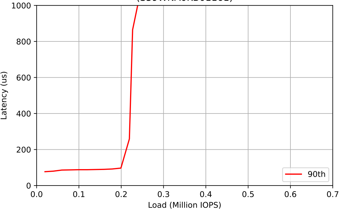
Workload: 750% Writes (S39WNA0KB01161)
