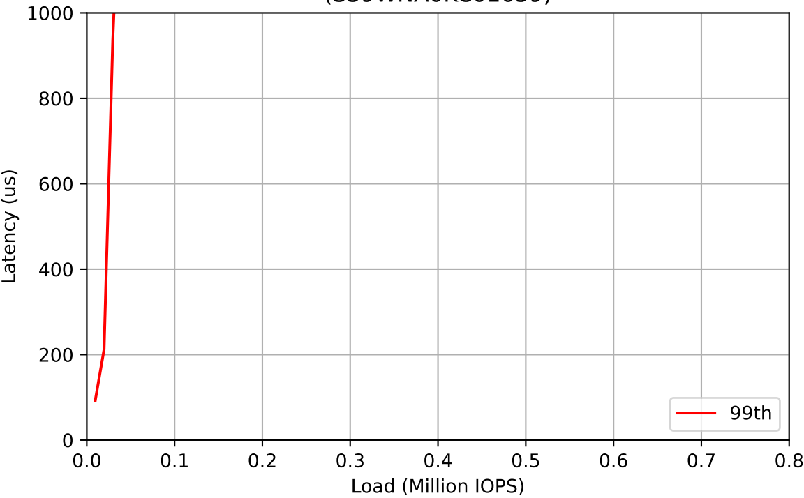
Workload: 500% Writes (S39WNA0KC01659)
