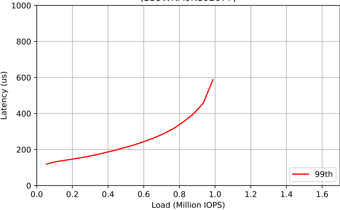
Workload: 100% Reads (S39WNA0KC02077)
