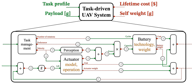
Fig. 4: Co-design diagram for a task-driven UAV, decomposed into functional components; designs carry implementation color. Red and green lines leaving the lower diagram are the four system-level functionalities/resources of the interface above.
