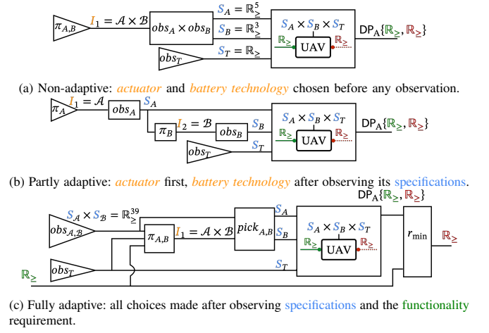
Fig. 7: Design processes for the UAV with different adaptivity levels.
