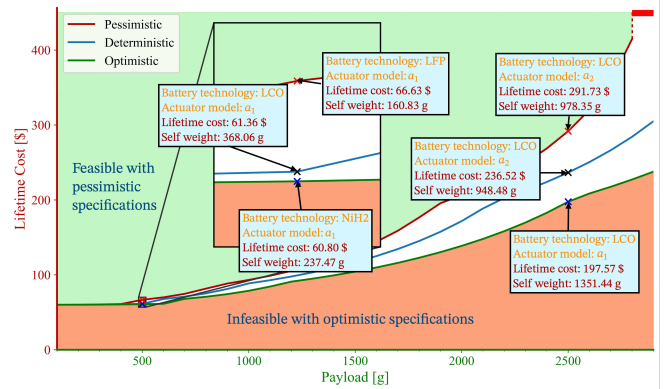
Fig. 5: Required payload versus minimal lifetime cost for a fixed task profile , deterministic and interval-uncertain. Pairs above the pessimistic curve (green) are robustly feasible, below the optimistic one (orange) infeasible even optimistically; between them, feasible for some realizations only. Labels give optimal implementations at some payloads; for large payloads the pessimistic model is infeasible, with minimal cost +\infty .
