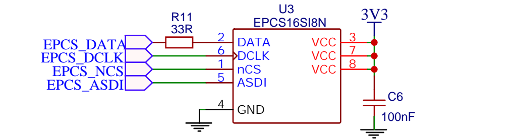
FPGA configuration memory chip
