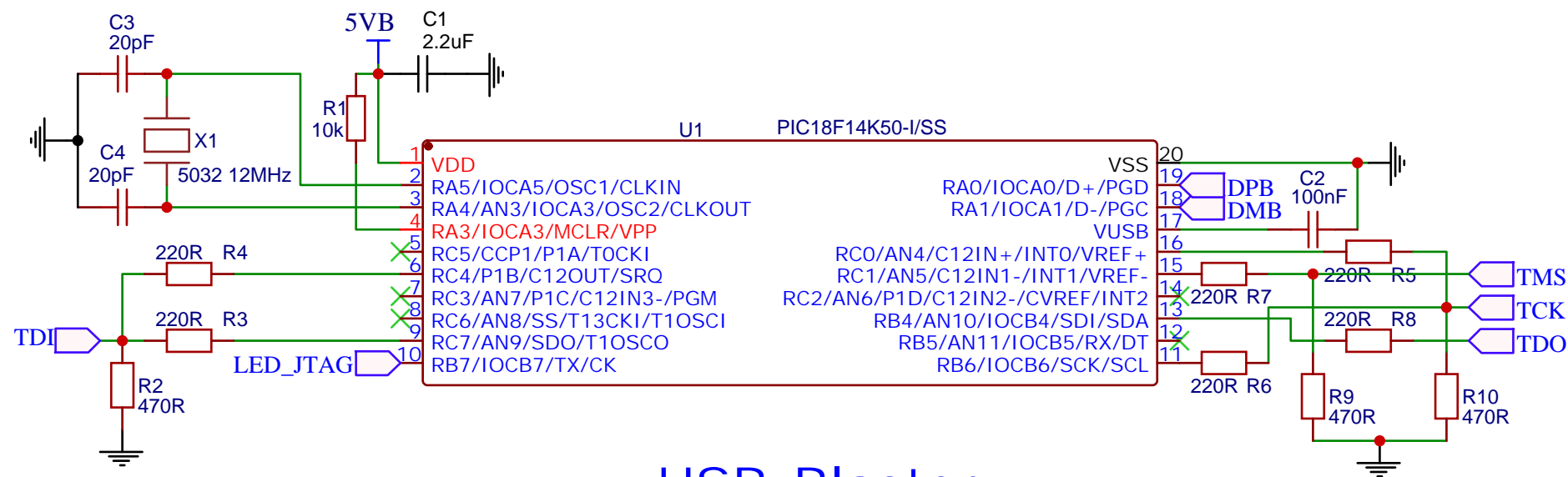
USB-Blaster
