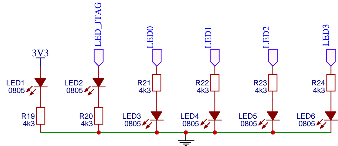
LED indicator
