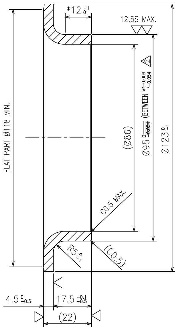
SECTION VIEW
