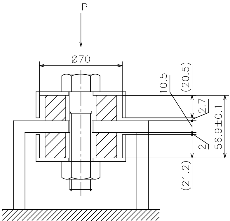
ASSEMBLY METHOD (SCALE: FREE)
