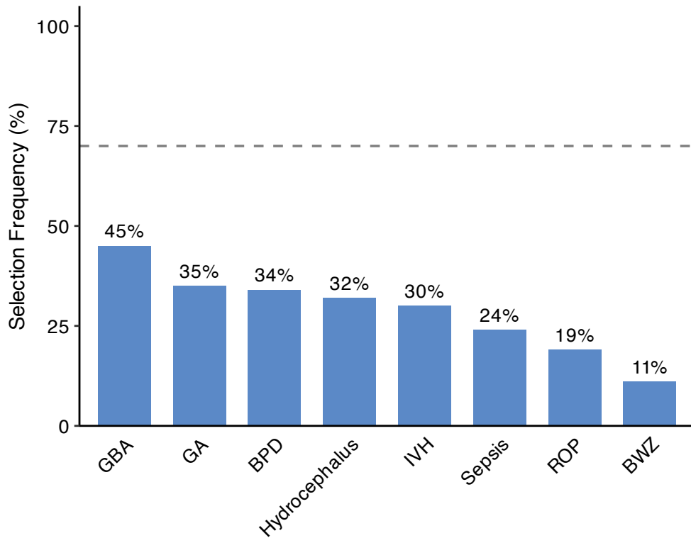
A. ACC stability selection (high-GBA removed)
