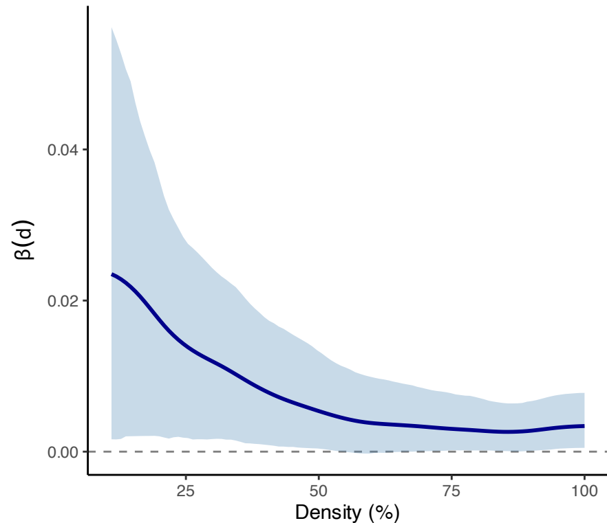
B. GBA effect on ACC (high-GBA removed)
