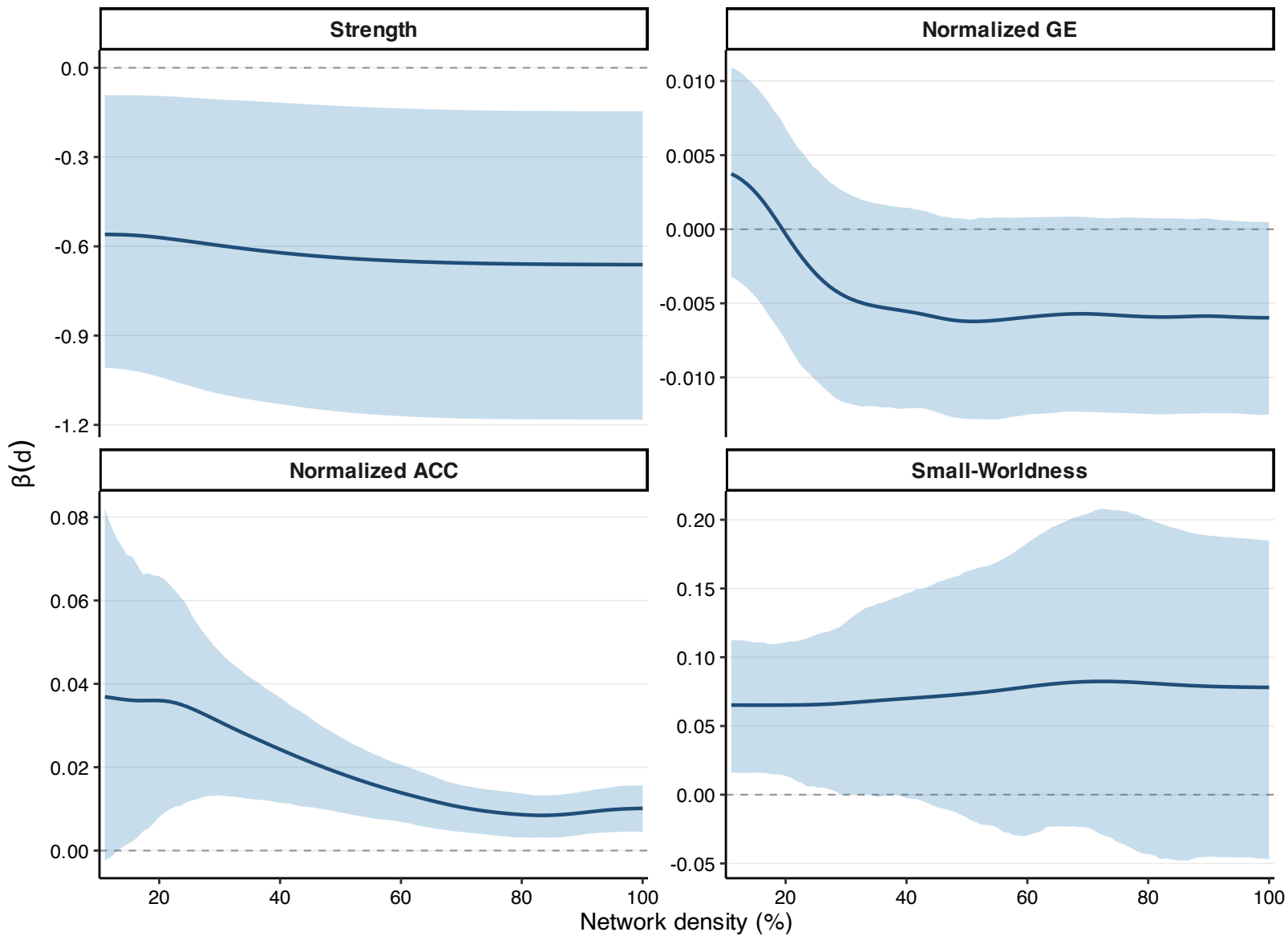
Supplementary Figure 6. Unadjusted group beta(density) curves
