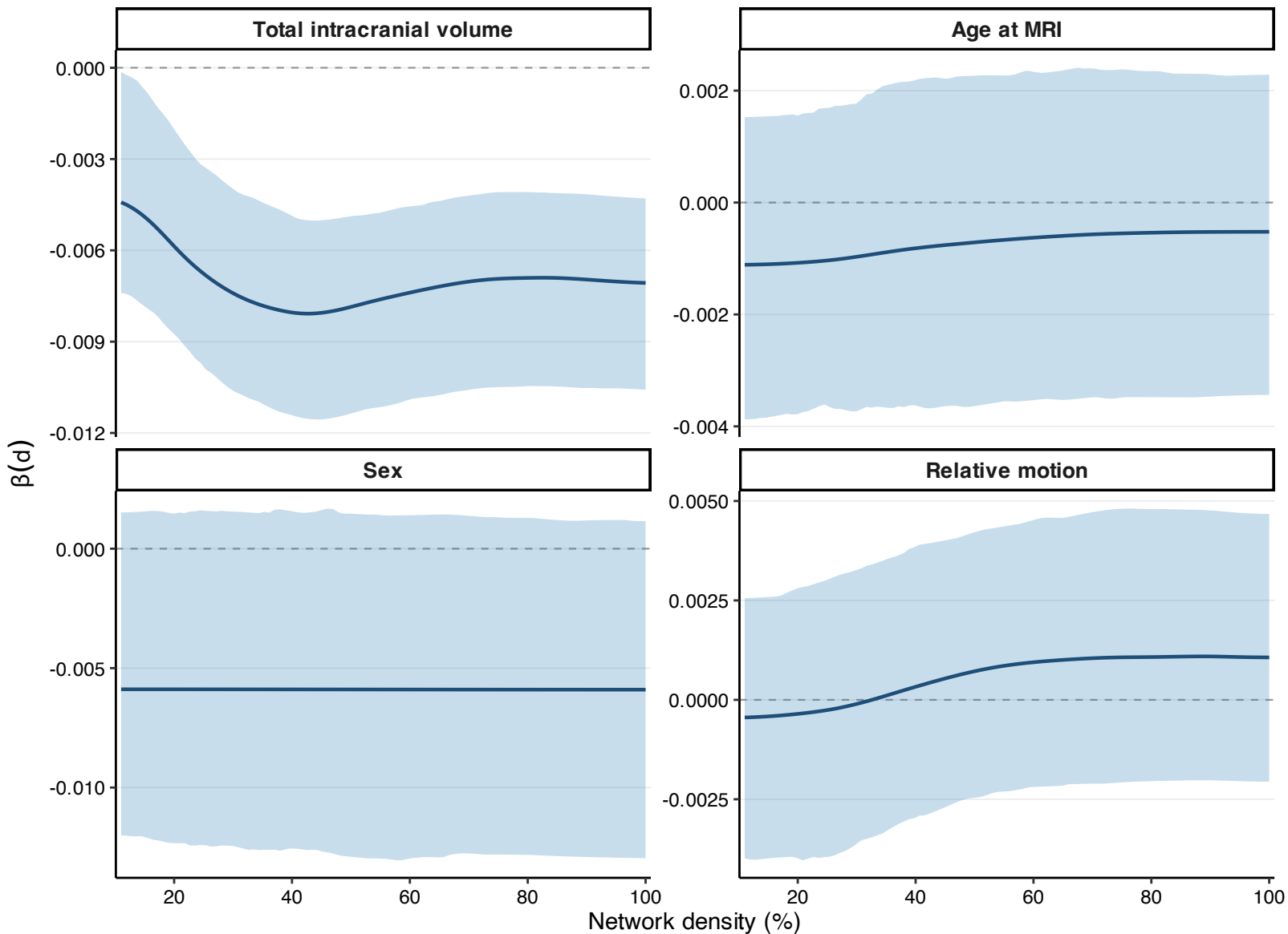
Supplementary Figure 8. Covariate beta(density) curves: Normalized GE
