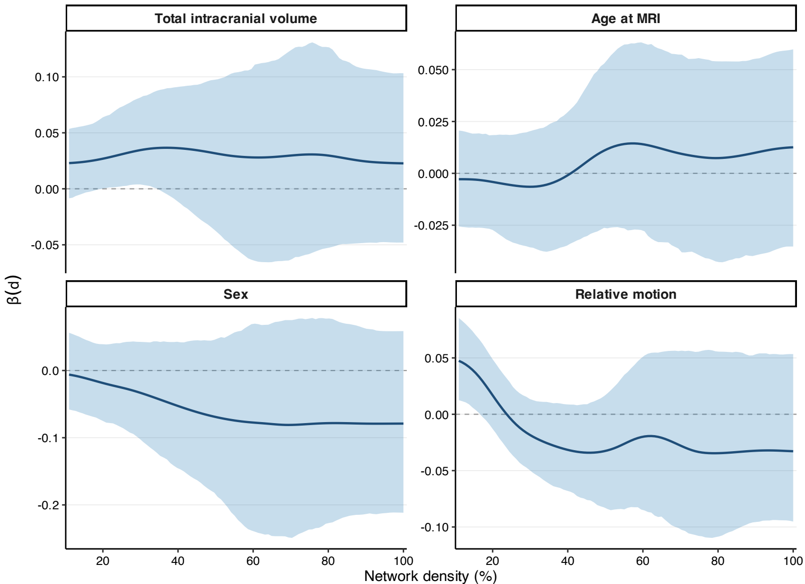
Supplementary Figure 10. Covariate beta(density) curves: Small-Worldness
