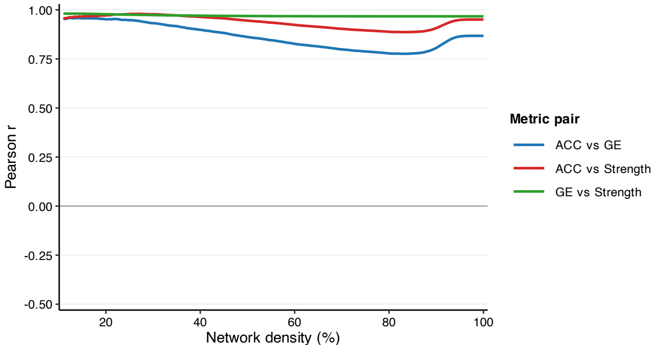
Supplementary Figure 1. Pre-normalization metric correlations across density
