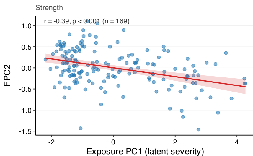
D. FPC2 vs. PC1
