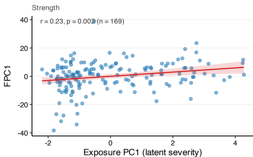
C. FPC1 vs. PC1
