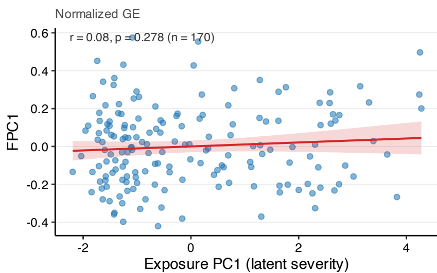
E. FPC1 vs. PC1
