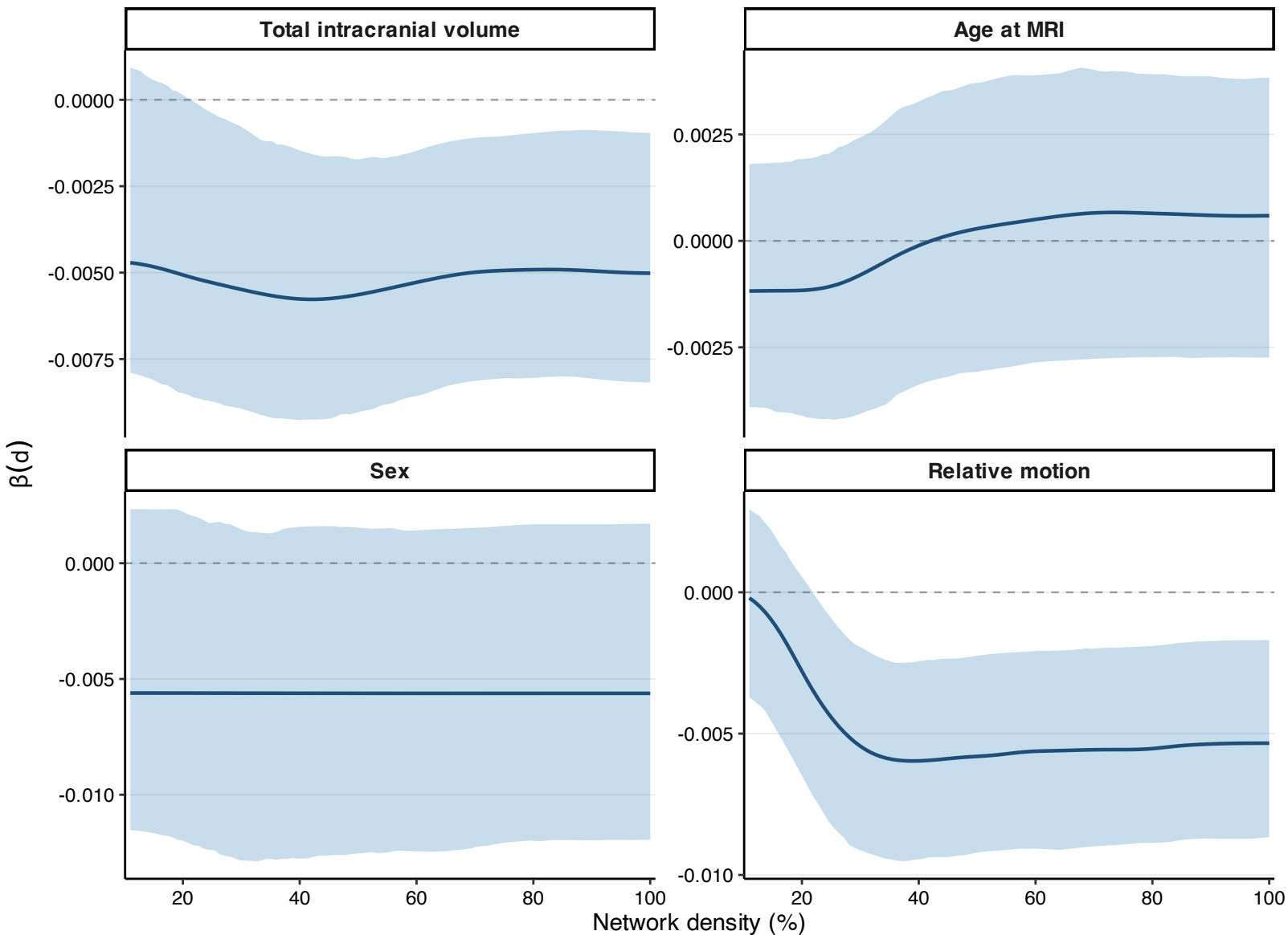
Supplementary Figure 7. Covariate beta(density) curves: Normalized GE
