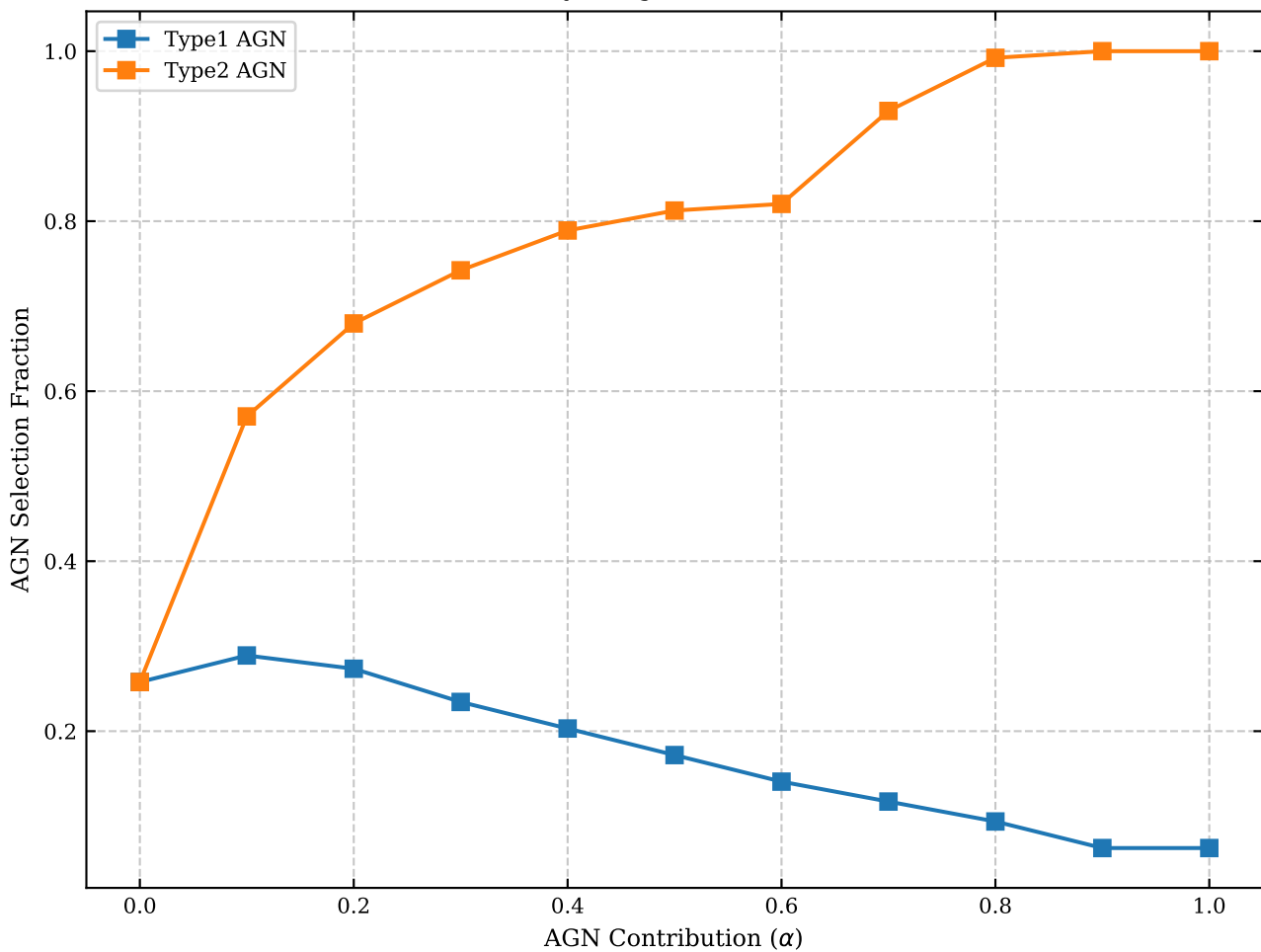
IRAC Lacy Wedge AGN Identification
