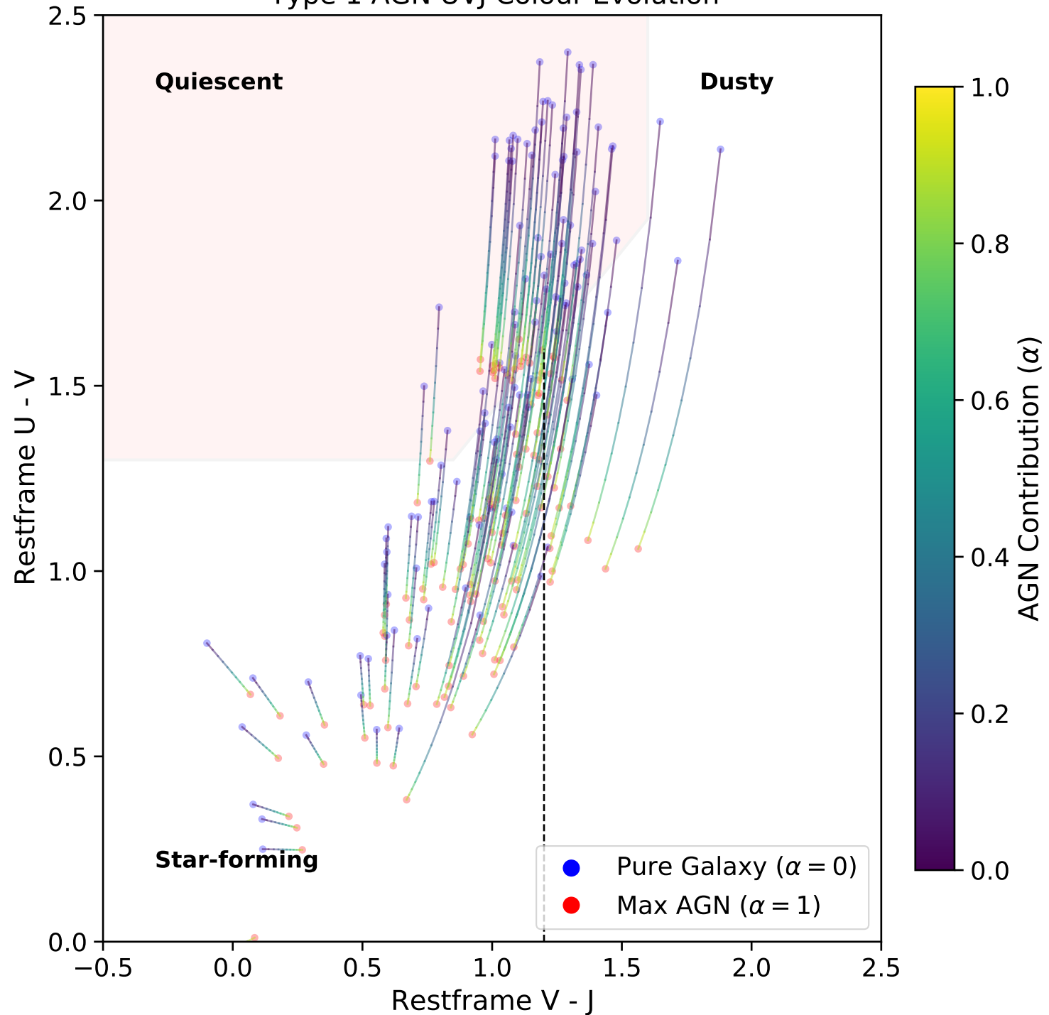
Type 1 AGN UVJ Colour Evolution
