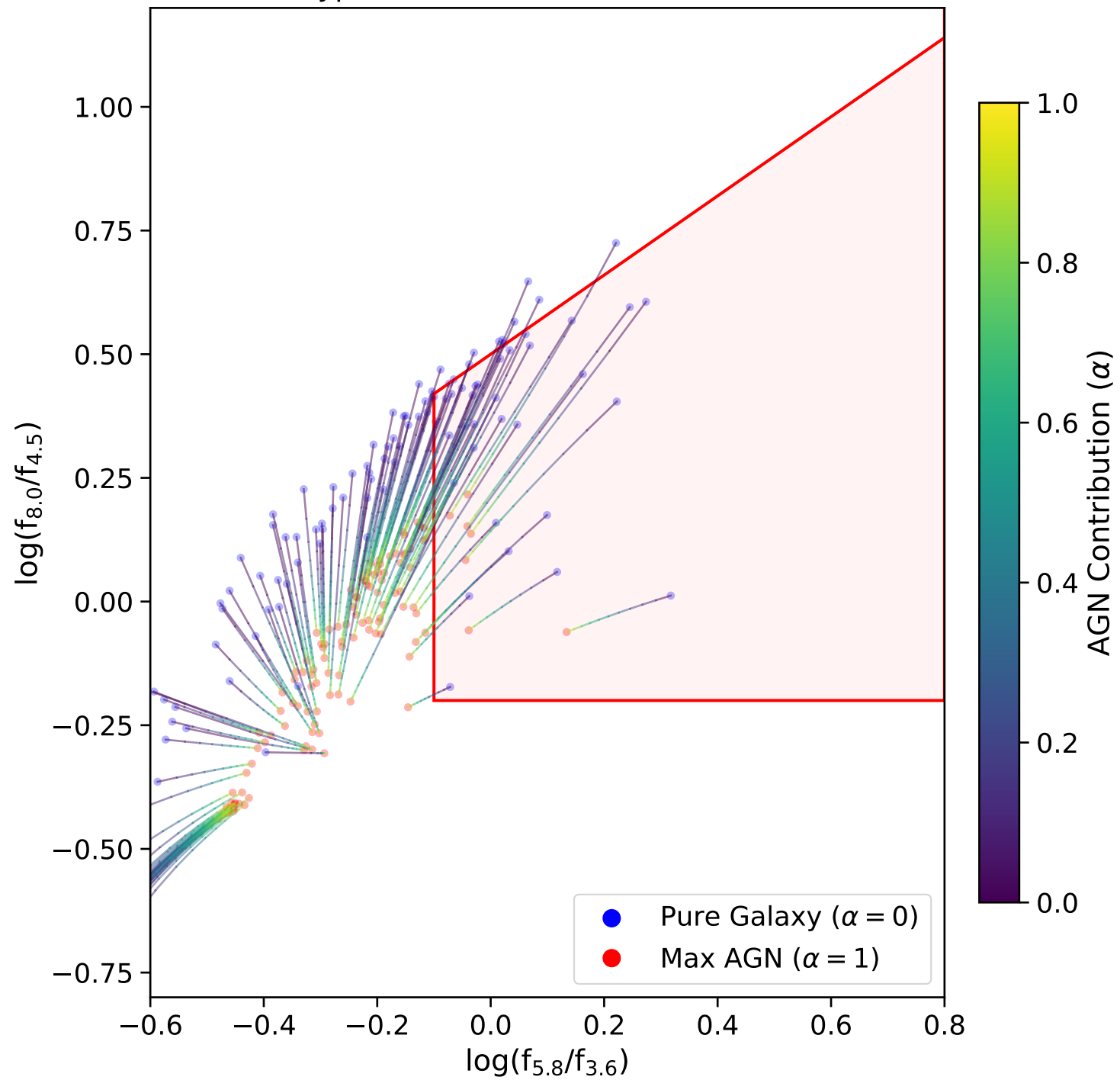
Type 1 AGN IRAC Colour Evolution
