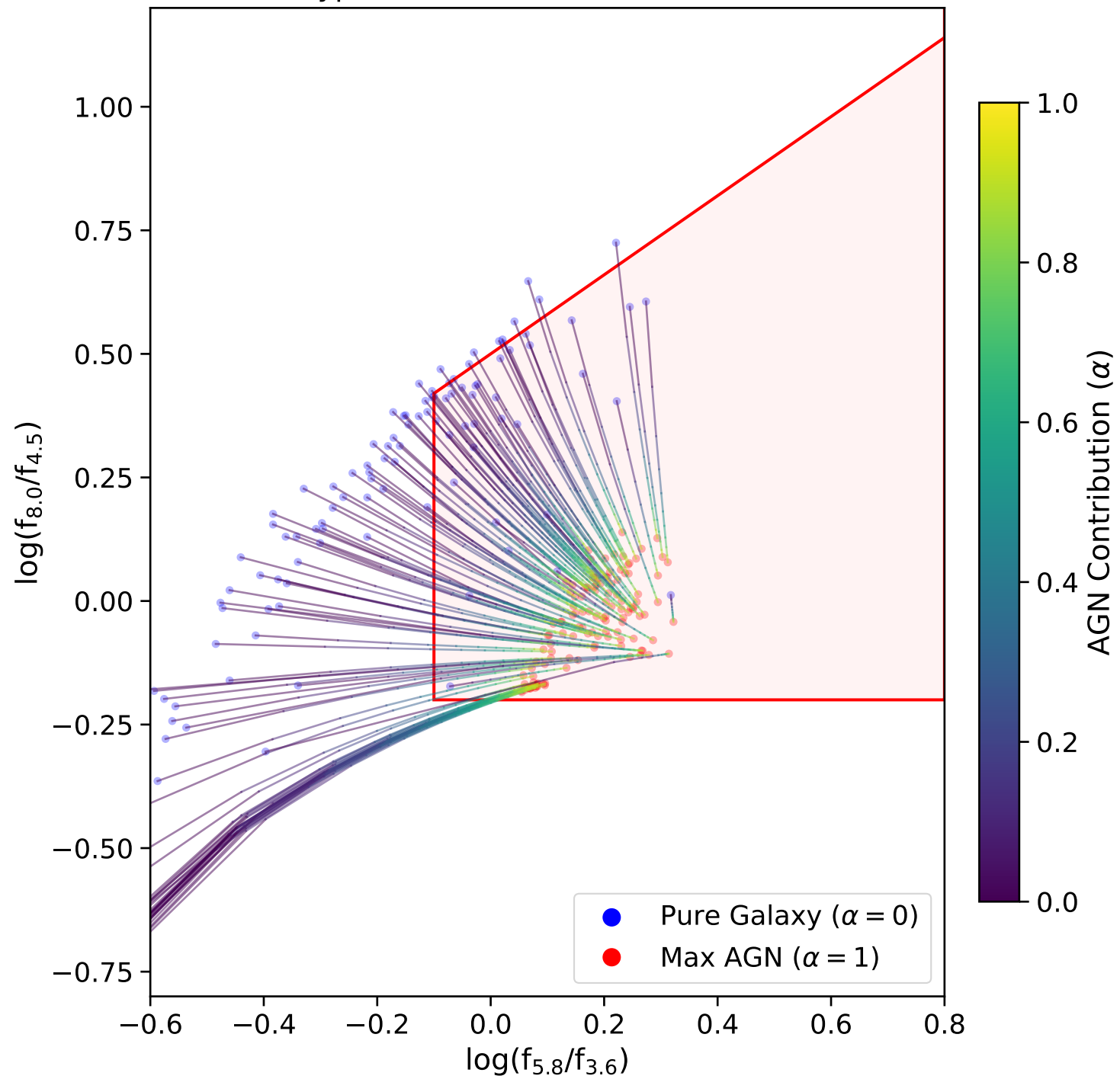
Type 2 AGN IRAC Colour Evolution
