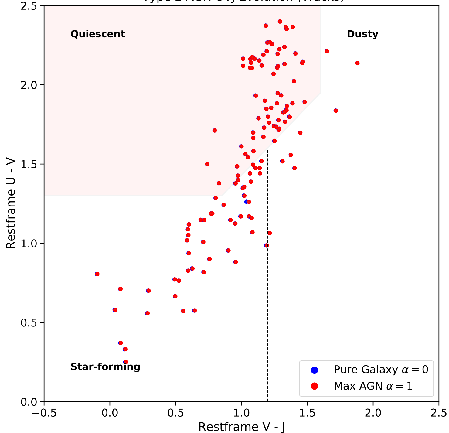
Type 2 AGN UVJ Evolution (Tracks)
