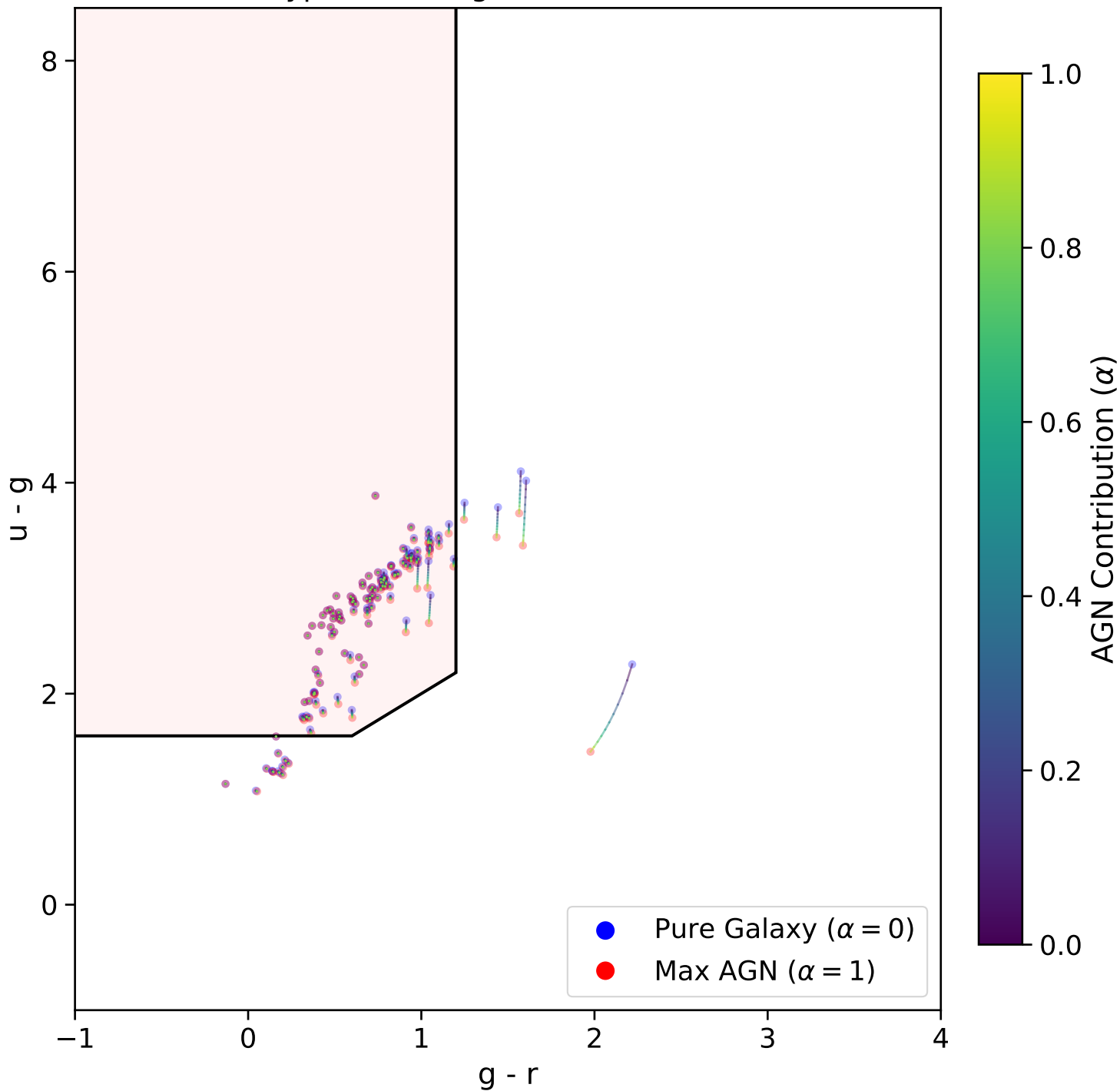
Type 2 AGN ugr Colour Evolution
