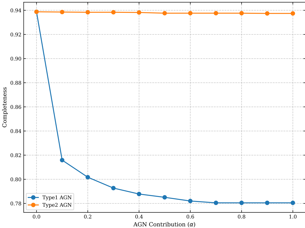
ugr Dropout Selection Completeness
