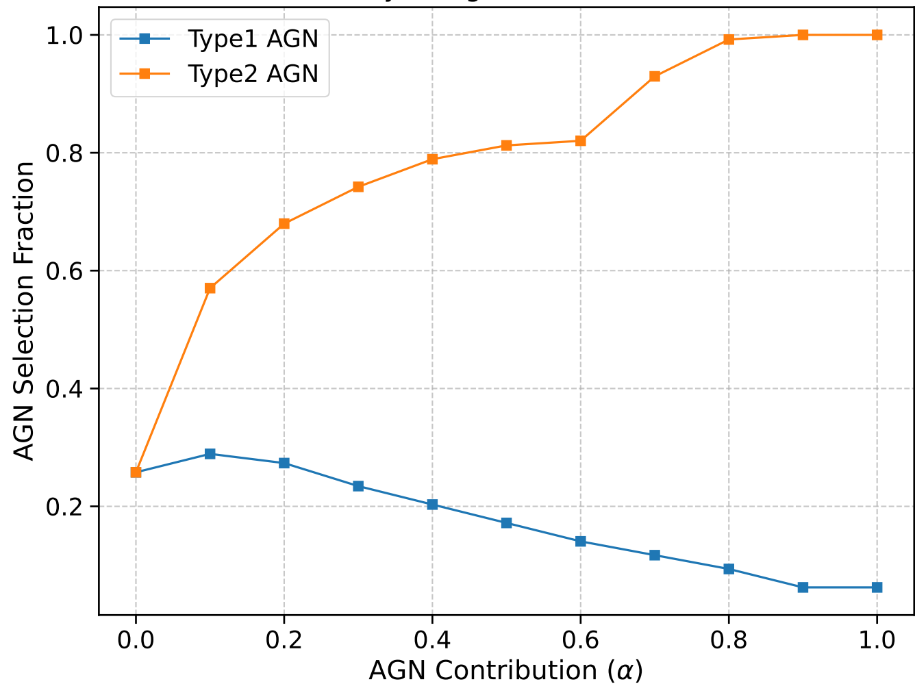
IRAC Lacy Wedge AGN Identification
