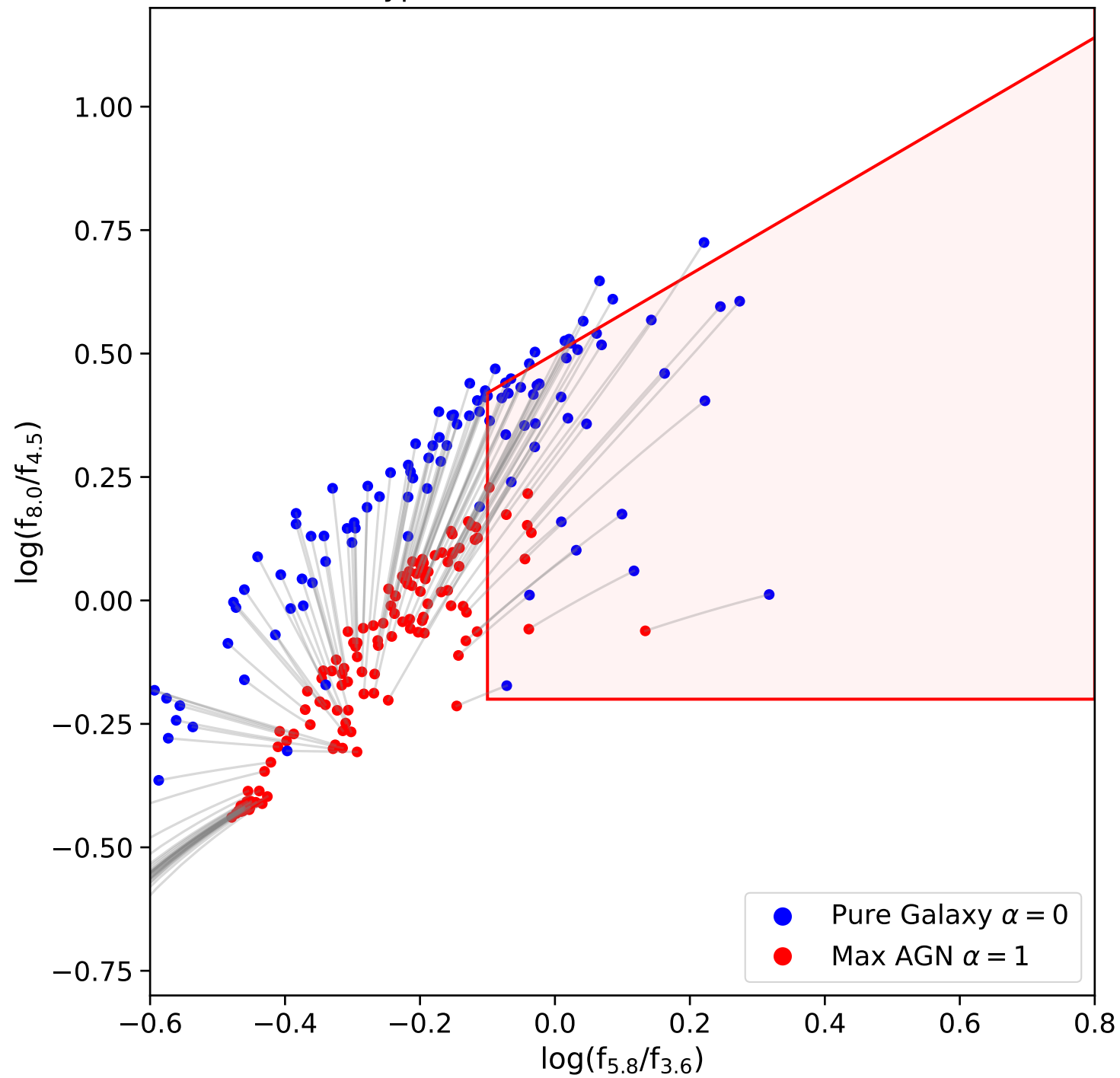
Type 1 AGN IRAC Evolution (Tracks)
