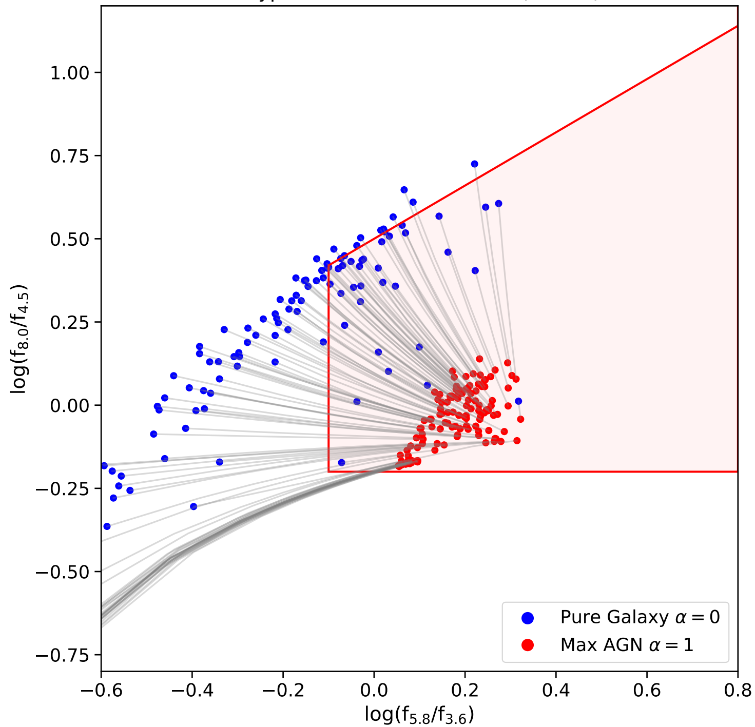
Type 2 AGN IRAC Evolution (Tracks)
