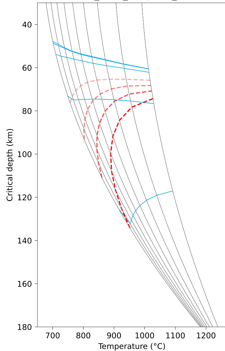
mackwell_1998_maryland_diabase
