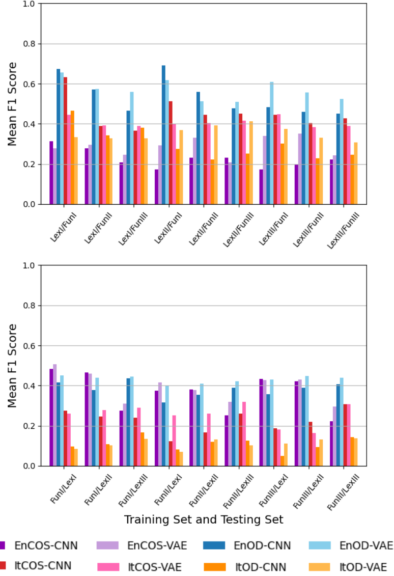
Figure 7: Mean F1 scores - training on LEX, testing on FUN (higher panel) and training on FUN, testing on LEX (lower panel) for each dataset and architecture.
