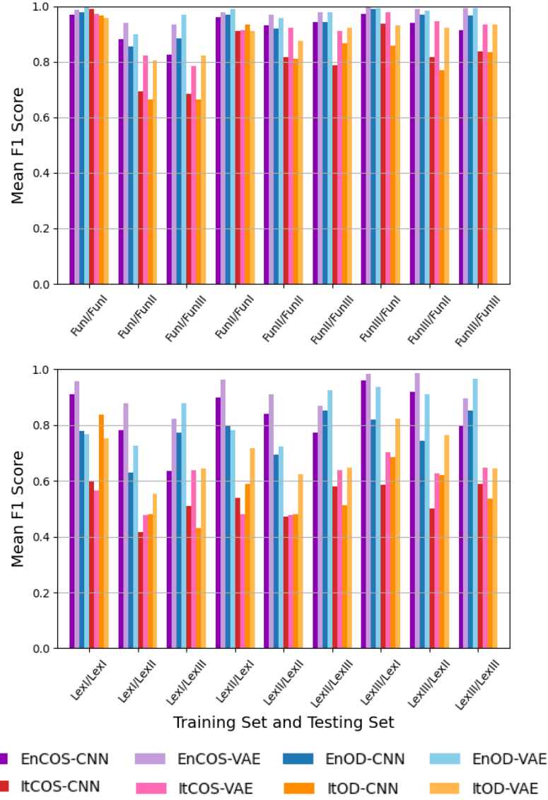
Figure 6: Training and testing across levels of abstractions in Fun (higher panel) and Lex (lower panel) in each dataset and architecture
