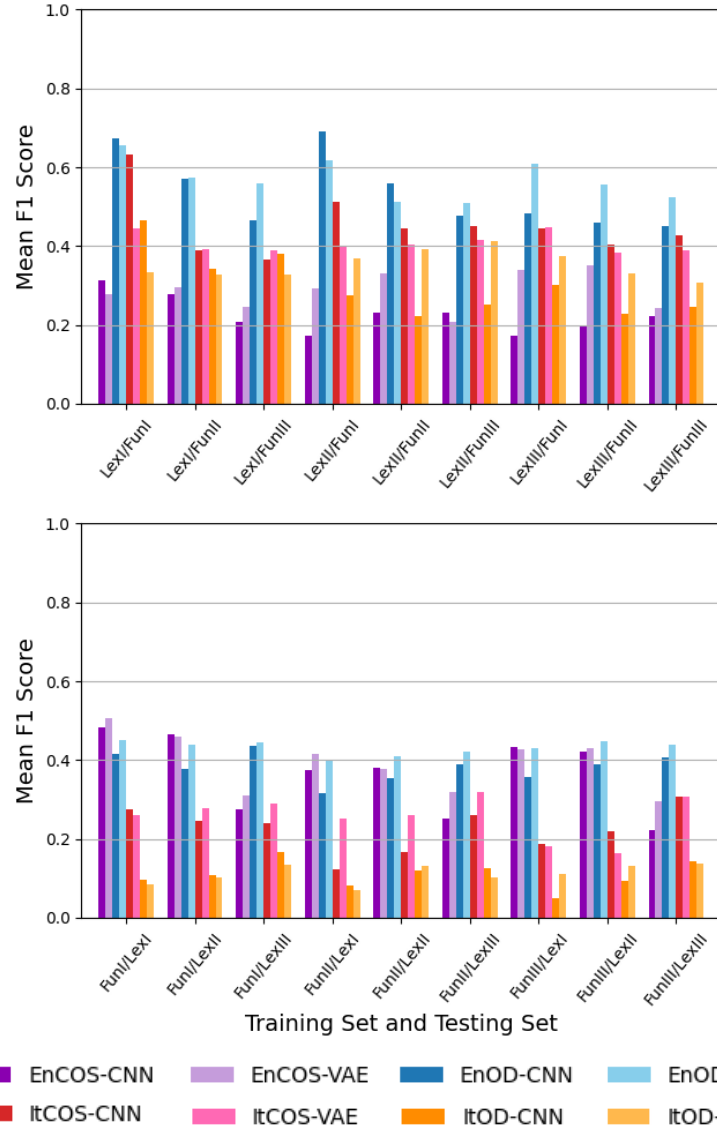
Figure 7: Mean F1 scores - training on LEX, testing on FUN (higher panel) and training on FUN, testing on LEX (lower panel) for each dataset and architecture.
