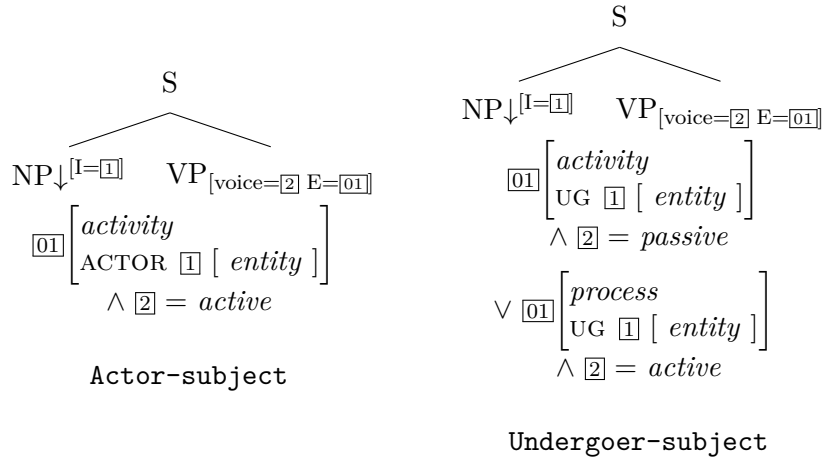
Figure 13: Subject linking for active and passive
