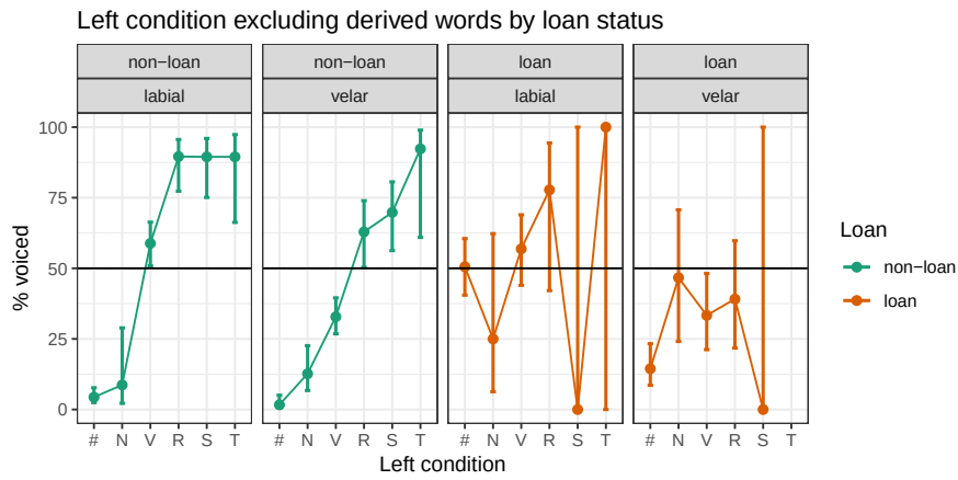
Fig. A2 Estimates of a logistic regression model with three predictors, LEFT CONDITION, PLACE, and LOAN with all interactions (derived words excluded).
