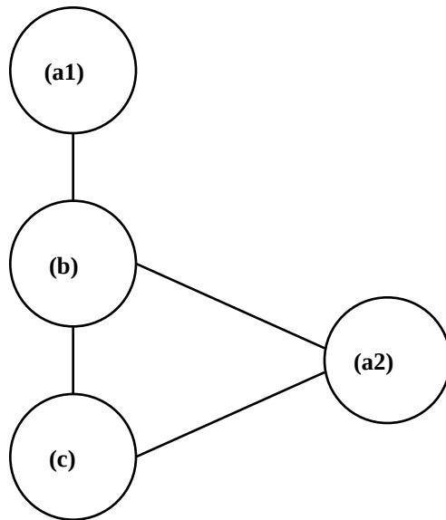
Figure A1. Diagram illustrating the structural relationship between primordial being (a1), the separated negation state (a2), and the dynamic interplay of forces (b, c). Adapted from Bissell and Levenstein (2011).
