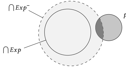
Figure 2: Minimality of \text{Exp}
