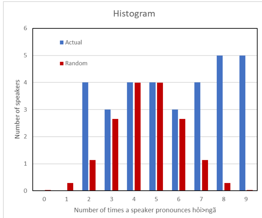
Figure 17. Blue columns: Histogram of number of times (n) each subject pronounces hoi>ngã. Red columns: histogram for non-differentiator subpopulation, obtained by fitting a binomial distribution to the central peak at n = 4 and 5 .
