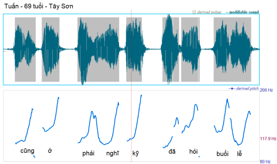
Figure 7. Pitch contour in a sentence (Tuấn, 69, Tây Sơn). Praat parameters as previous.
