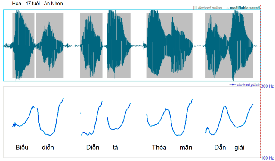
Figure 12. Pitch contour for composite words(Hoa, 47, An Nhon). Praat analysis parameters as previous.
