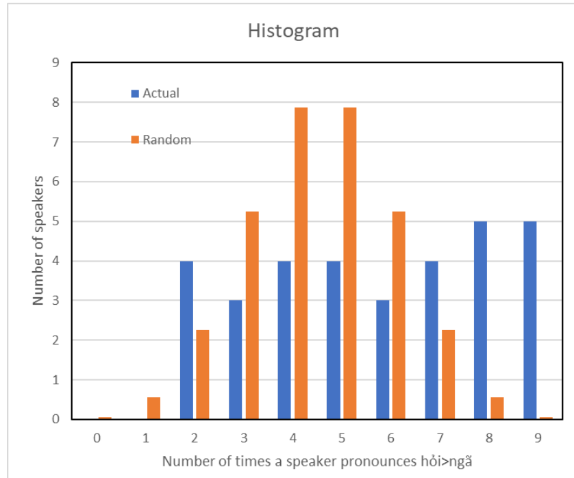
Figure 16. Blue columns: Histogram of number of times (n) each subject pronounces hoi>ngã. Orange columns: expected histogram if the results were completely random, i.e. nobody makes consistent tonal distinction (binomial distribution).
