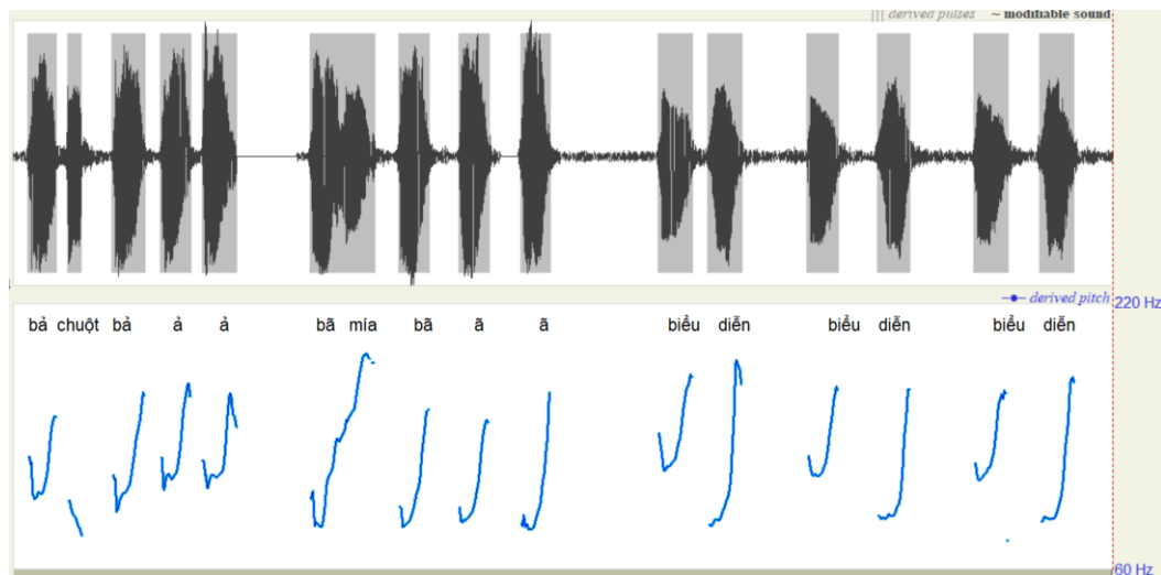
Figure 14. Repeatability of tones within word groups.
