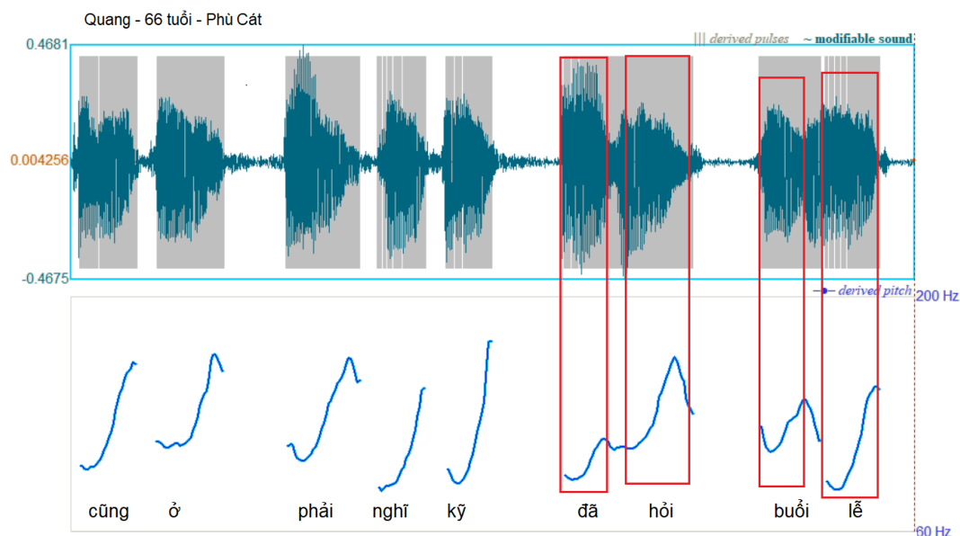
Figure 4. Pitch contour of words in sentence (Quang, 66, Phù Cát). Praat settings as previous.
