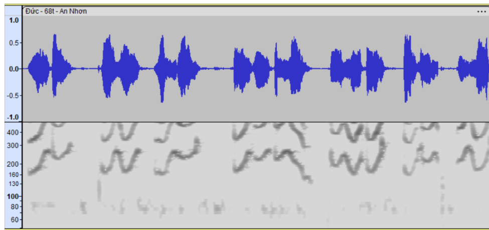
Figure 1: Spectrogram obtained with Audacity, showing the bands for F0 and F1.
