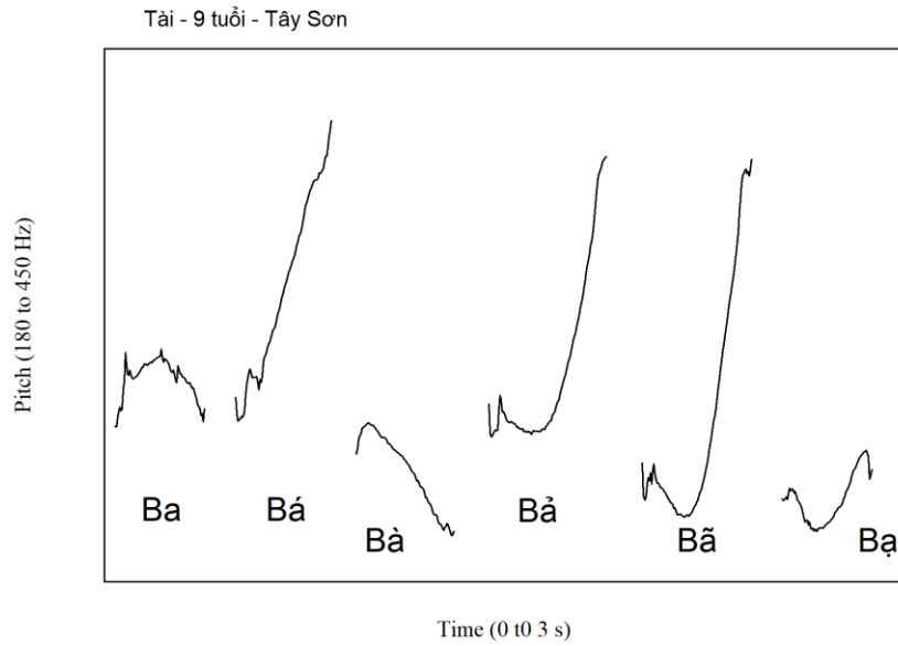
Hình 8. Độ cao (pitch contour) “ba bá bà bả bã bã bạ” (Tài, 9 tuổi, Tây Sơn) Pitch analysis parameters: raw autocorrelation method with floor 180 Hz, ceiling 450 Hz, silence threshold 0.03, voicing threshold 0.45, octave cost 0.01, octave jump cost 1.0, voiced / unvoiced cost 0.14.
