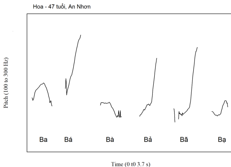
Figure 11. Pitch contour of “ba bá bà bả bã bạ” (Mrs Hoa, 47, An Nhơn). Praat pitch analysis parameters: raw autocorrelation method with floor 100 Hz, ceiling 300 Hz, silence threshold 0.05, voicing threshold 0.3, octave cost 0.01, octave jump cost 1.0, voiced / unvoiced cost 0.14.
