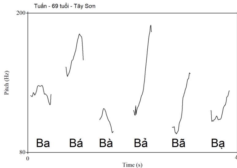
Hình 5. Độ cao (pitch contour) “ba bá bà bả bã bạ” (ông Tuấn, 69 tuổi, Tây Sơn) dùng Praat. Pitch analysis parameters: raw autocorrelation method with floor 80 Hz, ceiling 200 Hz, silence threshold 0.03, voicing threshold 0.45, octave cost 0.01, octave jump cost 1.0, voiced / unvoiced cost 0.14.
