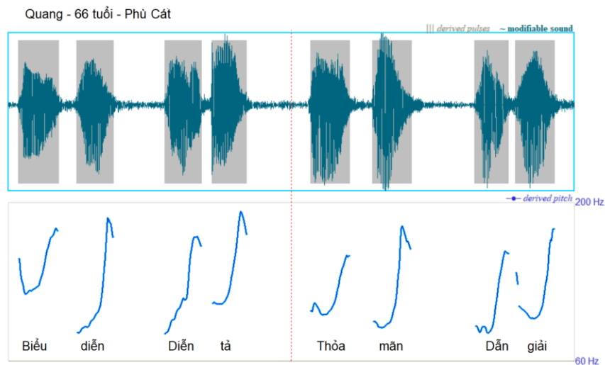
Figure 3. Pitch contour of composite words (Quang, 66, Phù Cát). Praat settings as previous.
