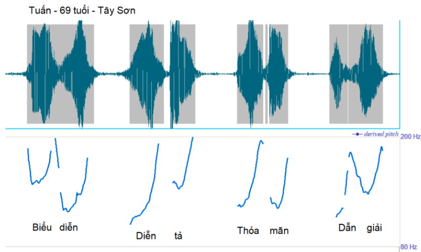
Figure 6. Pitch contour of composite words (Tuấn, 69, Tây Sơn). Praat parameters as previous.
