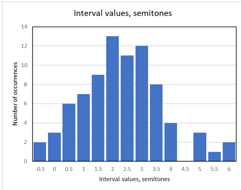
Figure 18. Histogram of hỏi ngã interval values in the 10 best differentiators. Each column represents the number of occurrences of hỏi-ngã intervals within \pm 0.25 of the x-axis label value.
