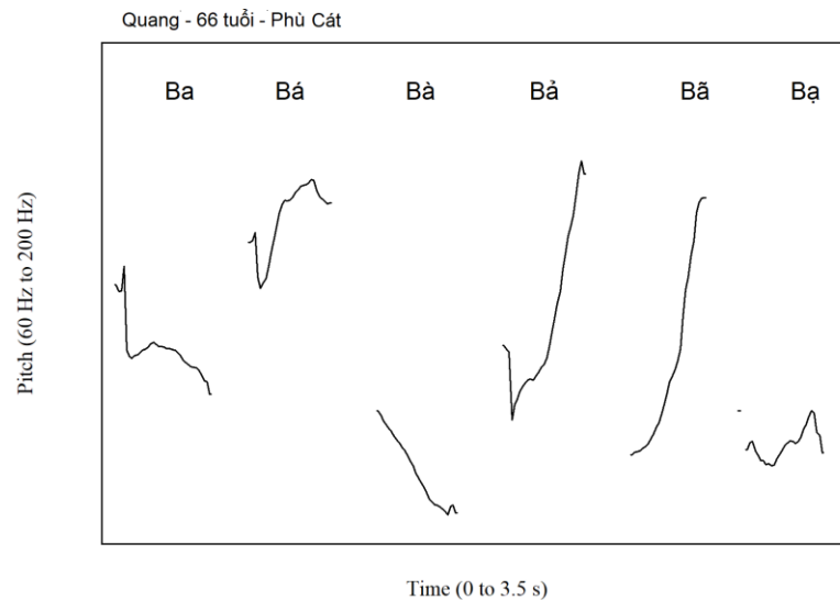
Figure 2. Pitch contour of “ba bá bà bả bã bã bạ” (Quang, 66, Phù Cát) using Praat. Pitch analysis parameters: raw autocorrelation method with floor 60 Hz, ceiling 200 Hz, silence threshold 0.1, voicing threshold 0.4, octave cost 0.1, octave jump cost 1.0, voiced / unvoiced cost 0.14.
