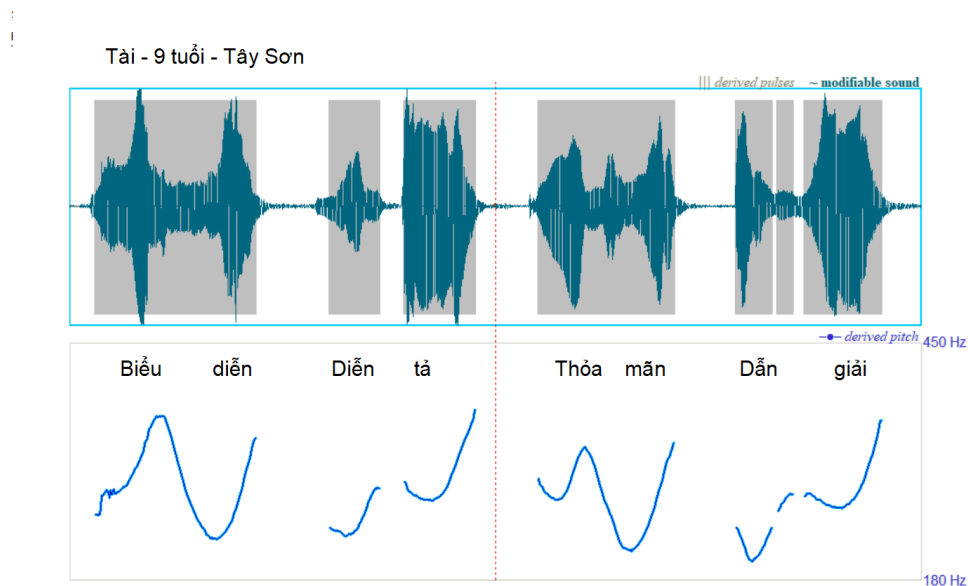
Figure 9. Pitch contour of composite words (Tài, 9, Tây Sơn). Praat analysis parameters as previous.
