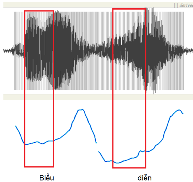
Figure 15. Using the average pitch of the first half vowel to compare hỏi and ngã.
