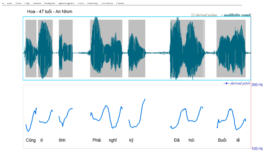
Figure 13. Pitch contour for words in a sentence (Hoa, 47, An Nhon). Praat analysis parameters as previous.
