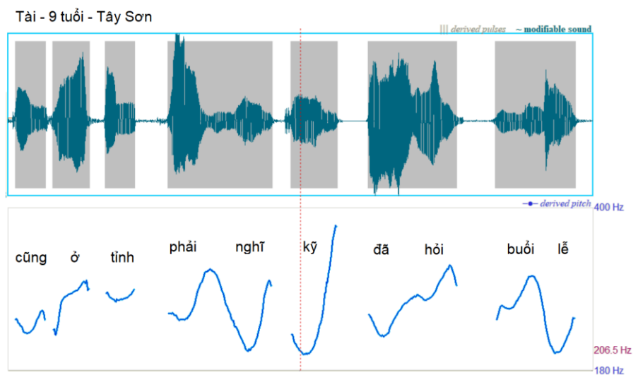
Figure 10. Pitch contour of words in a sentence (Tài, 9, Tây Sơn). Praat analysis parameters as previous.
