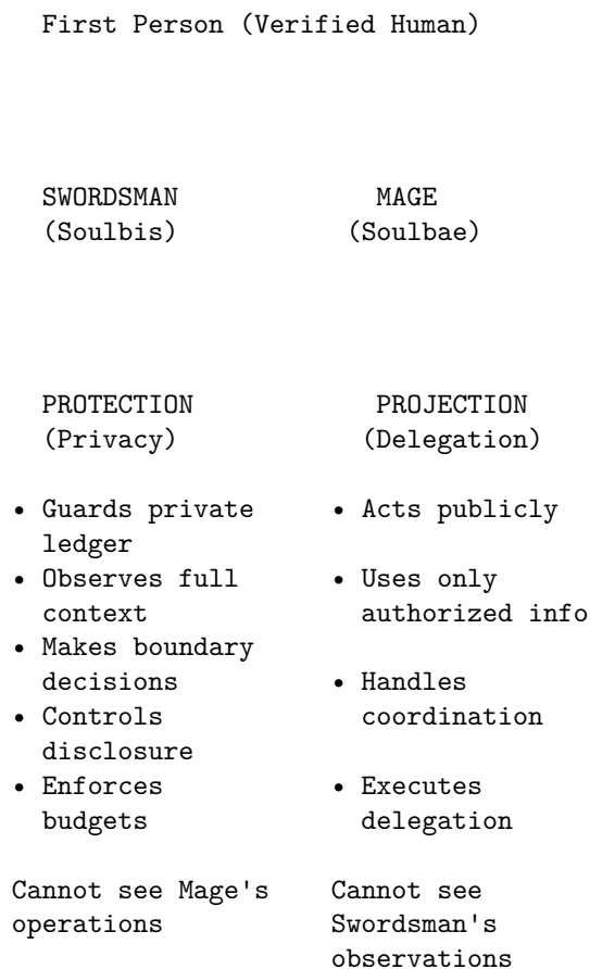
Figure 1: The Dual-Agent Architecture: Swordsman and Mage
