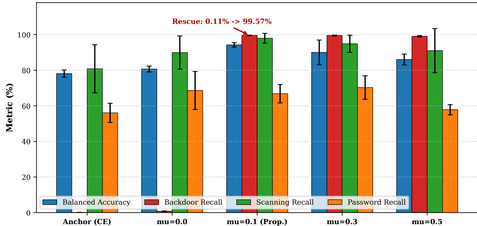
Performance Metrics Across SupCon Regularization Strength \mu (Mean \pm Std, 3 Seeds)
