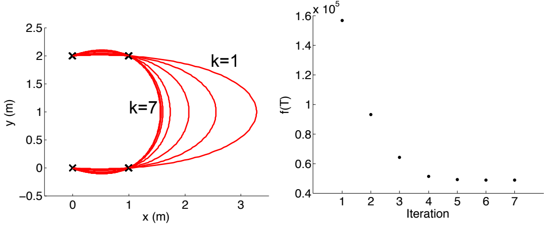
Figure 6.2: Illustration of relative time scaling. Left: Trajectory for different iterations. Right: Cost function vs. iteration.
