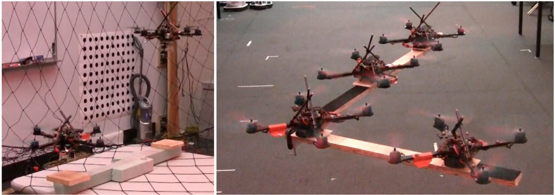
Figure 3.4: Left: Image from an experiment with the gripping mechanism enabling cooperative grasping, manipulation, and transportation. Right: Four quadrotors carrying a payload in the EI configuration. Videos of the experiments are available at http://tinyurl.com/penndars .
