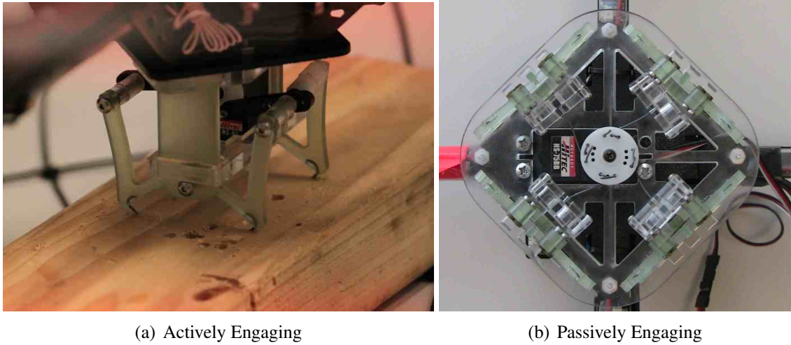
Figure 4.3: Ingressive Grippers
