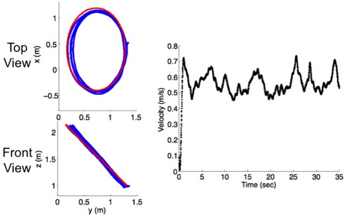
Figure 3.3: Trajectory tracking data for the Cross configuration along a 0.8, m radius circle tilted at 45^\circ from horizontal at 0.6 m/s.
